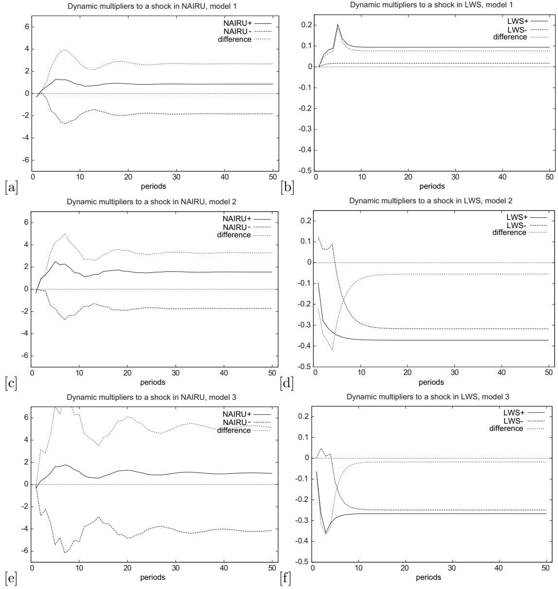
Figure 5: Dynamic multipliers
