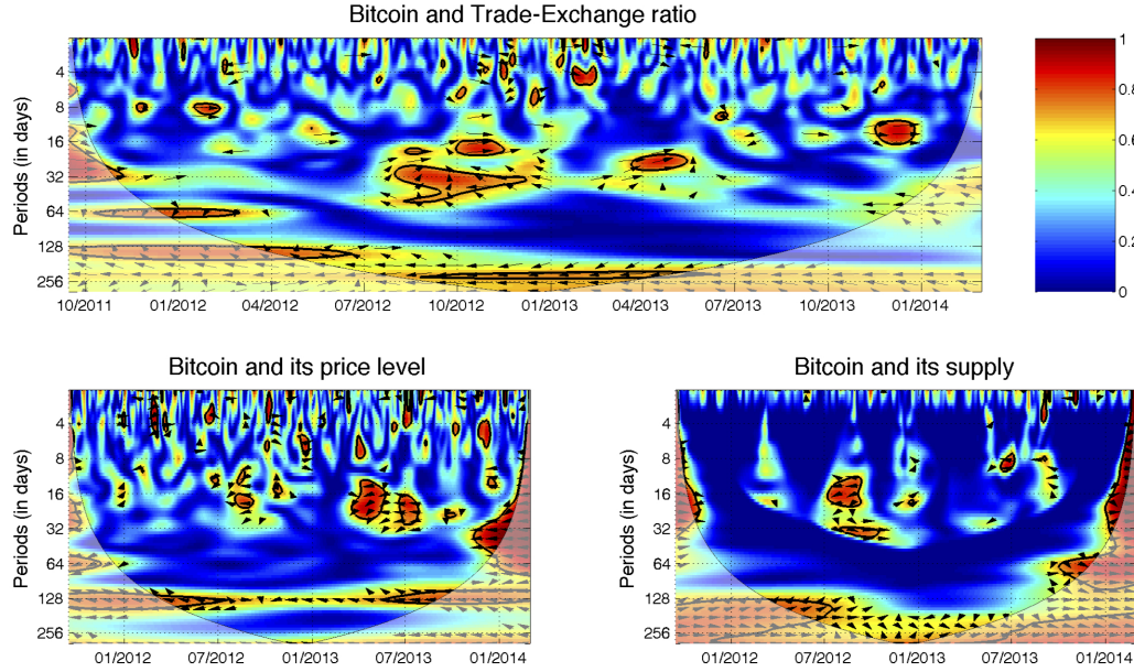
Figure 2. Fundamental drivers. Wavelet coherence is represented by a colored contour: the hotter the color is, the higher the local correlation in the time-frequency space (with time on the x -axis and scale on the y -axis). The matching of colors and correlation levels is represented by the scale on the right hand side of the upper graph. Regions with significant correlations tested against the red noise are contrasted by a thick black curve. The cone of influence separating the regions with reliable and less reliable estimates is represented by bright and pale colors, respectively. Phase (lag-lead) relationships are shown by the arrows – a positive correlation is represented by an arrow pointing to the right, a negative correlation by one to the left, leadership of the first variable is shown by a downwards pointing arrow and if it lags, the relationship is represented by an upward pointing arrow. The latter two relationships hold for the in-phase relationship (positive correlation); for the anti-phase (negative correlation), it holds vice versa. Henceforth, specifically for the fundamental drivers, Bitcoin price is negatively correlated to the Trade-Exchange ratio ( top ) over the long-term for the entire analyzed period, and there is no evident leader in the relationship. The Bitcoin price level is negatively correlated with the Bitcoin price in the long-term for the entire analyzed period as well ( bottom left ), with no evident leader. For the relatively calm period between 05/2013 and 09/2013, the price level led the prices in the medium term. The supply of bitcoins is positively correlated with the price in the long-term ( bottom right ), with no evident leader.
