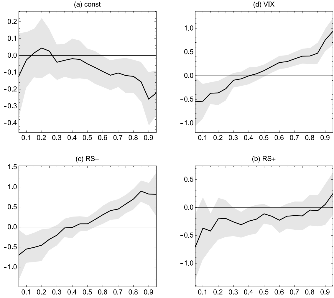
Figure 3: Estimated quantile regression process for model LQR3 in Table 4 for S&P 500 futures returns. For each \alpha -quantile ranging from 0.05 to 0.95, we plot the estimated parameters in the quantile regression ( \hat{\beta}(\alpha) ) together with pointwise 95% bootstrapped confidence intervals.
