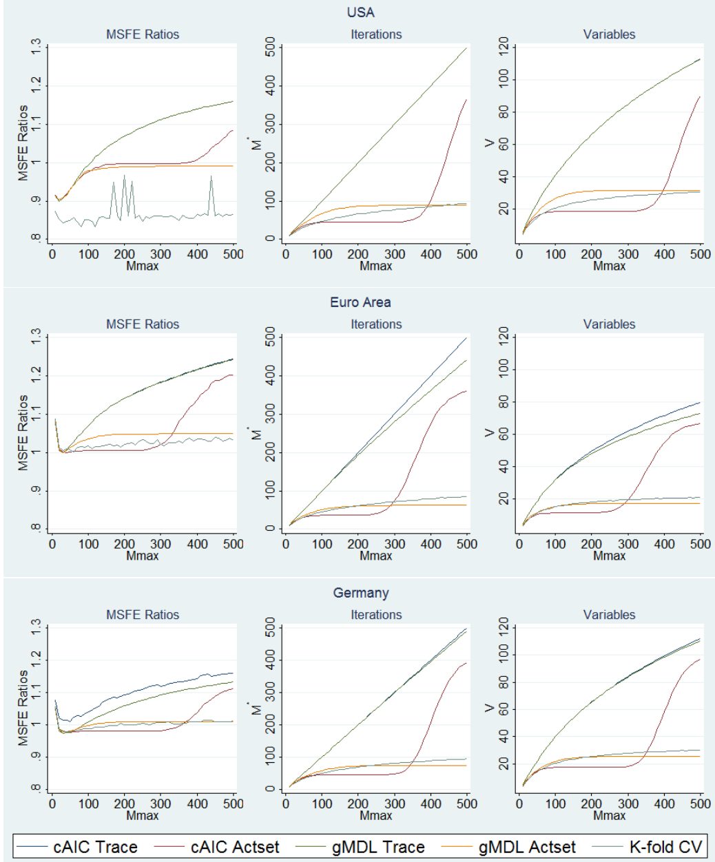
Figure 2: Comparison across Stopping Criteria
