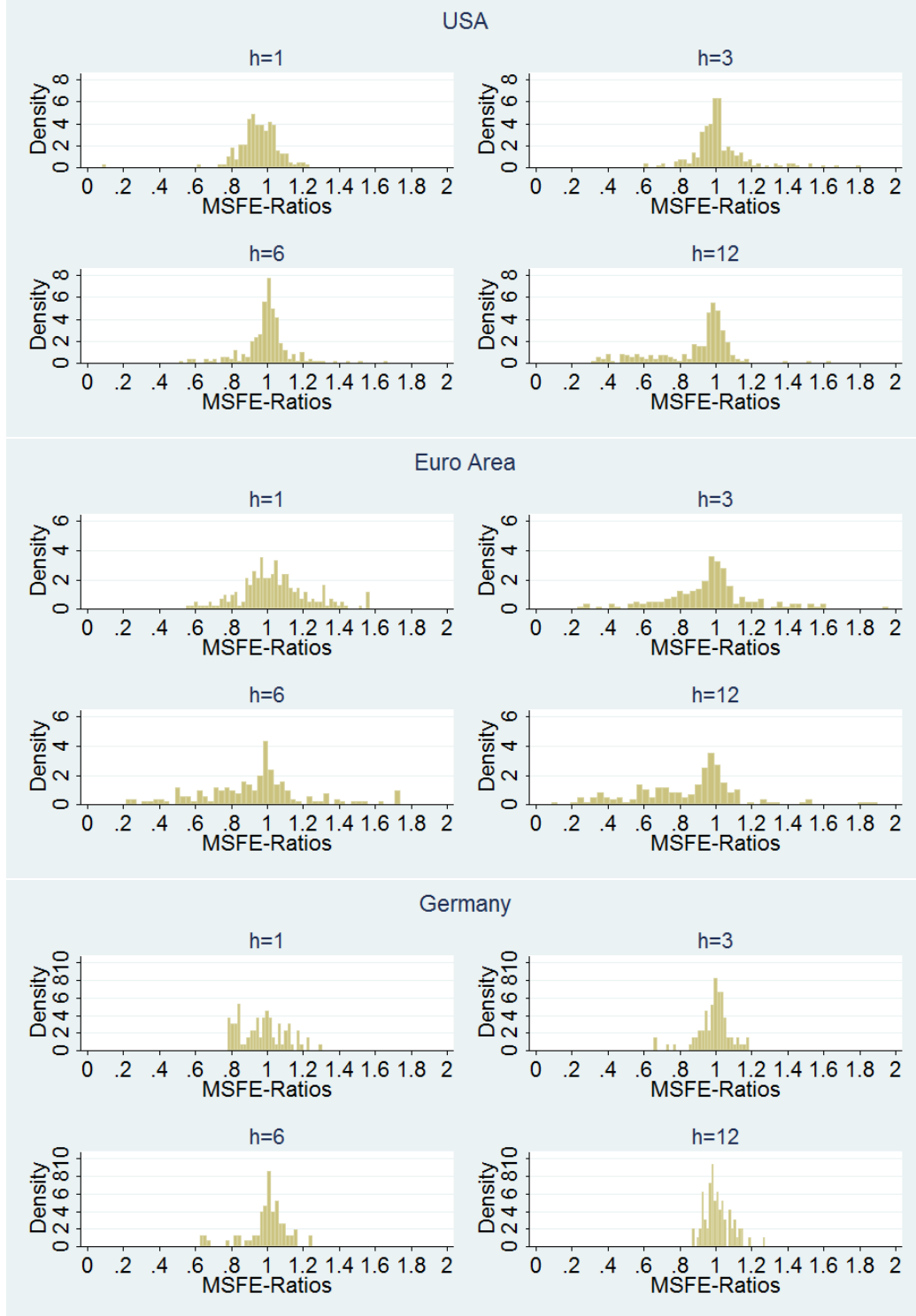
Figure 1: Histograms of MSFE-Ratios
