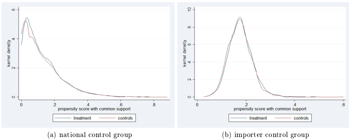
Figure 9: Distribution of matched propensity scores
