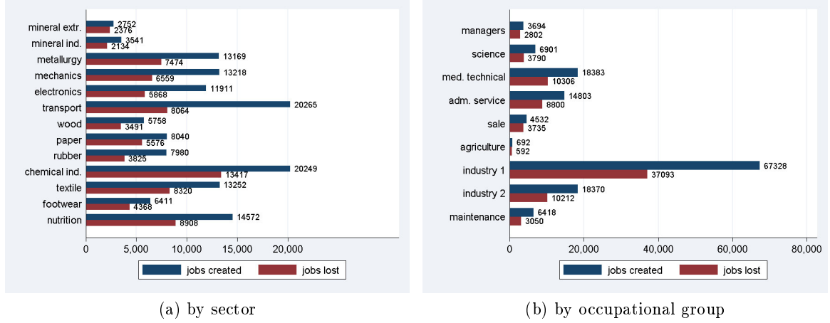
Figure 5: Distribution of won and lost jobs
