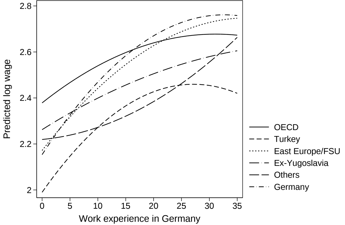
Fig. 1 Simulated assimilation profiles by area of origin (Males). It is assumed that natives obtained their education solely in Germany ( FYOS=0 , GYOS=12 ) and immigrants solely abroad ( FYOS=12 , GYOS=12 ). Further, immigrants have no foreign labor market experience ( FLX=0 ).
