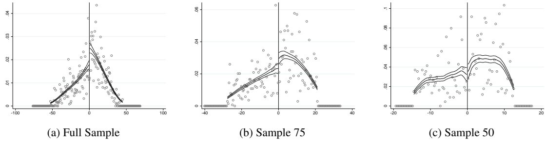
Figure 5: McCrary Test
