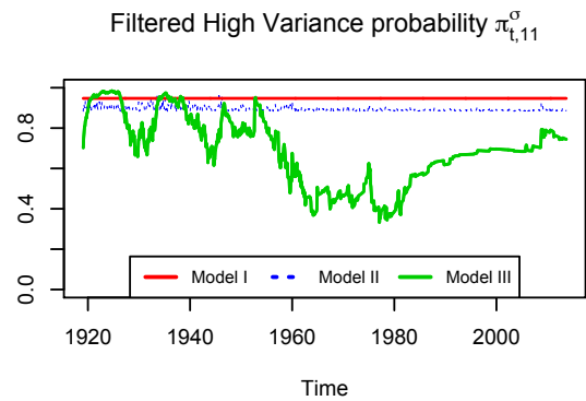
Figure 2: Smoothed probability estimates for the recession regime in the mean and for the high variance regime. Filtered transition probability estimates for the low and high variance regimes. In the first graph, the vertical gray areas indicate recessions according to the NBER business cycle classifications.
