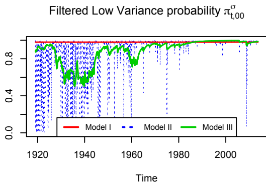
Figure 2: Smoothed probability estimates for the recession regime in the mean and for the high variance regime. Filtered transition probability estimates for the low and high variance regimes. In the first graph, the vertical gray areas indicate recessions according to the NBER business cycle classifications.
