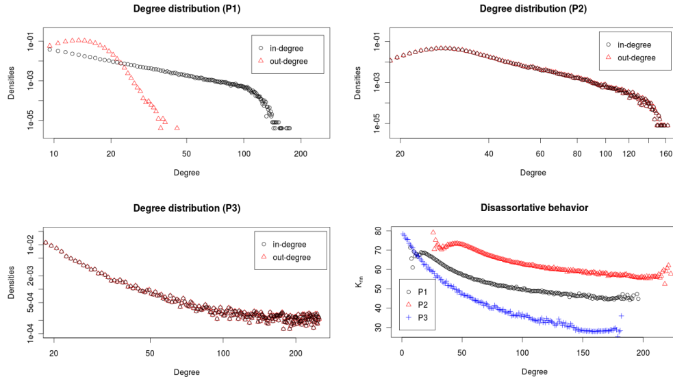
Fig. 2: The first three panels show the in- and out-degree distributions for the three probability functions (14), (15) and (16). The last panel shows the mean neighbour degree as a function of the total degree of the nodes. The curves in the last panel are decreasing with the degree itself, indicating that big nodes are connected to a multitude of small and medium-sized nodes, which themselves are connected with only a (relatively) small number of hubs.
