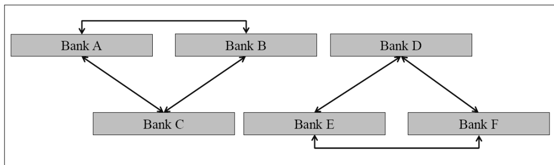
Figure 4: Clustered Subnetworks
