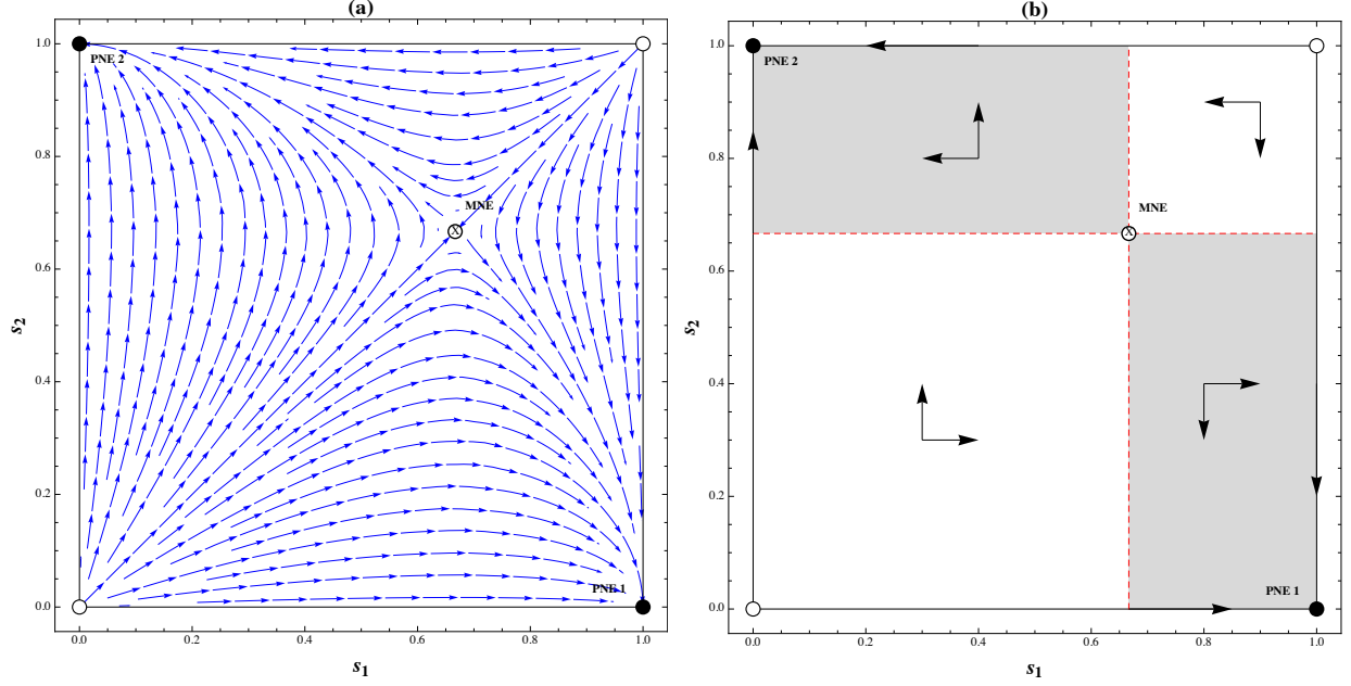
Figure 2: Dynamics for two populations. Phase portrait for replicator dynamics (Panel A), and differential inclusions for sign-preserving dynamics (Panel B). Shaded rectangles are absorbing while unshaded rectangles are transient under sign preserving dynamics.
