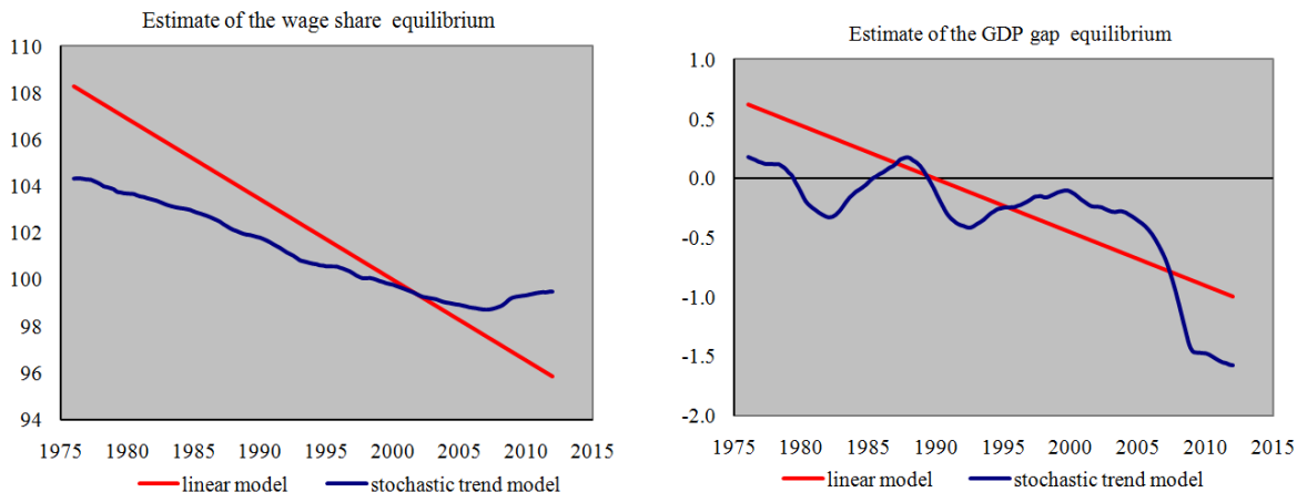
Figure 7: Comparing the linear and stochastic trend estimates of state variables
