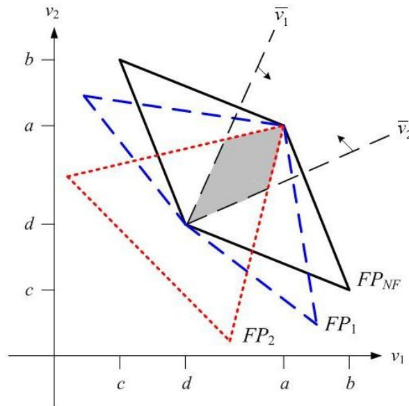
Figure 5. Effects of higher \alpha_i on the FIR set.
