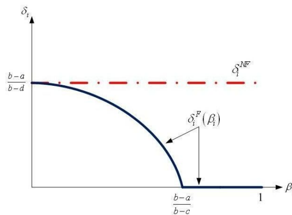
Figure 2. Discount factors \delta_i^F(\beta_i) and \delta_i^{NF} .
