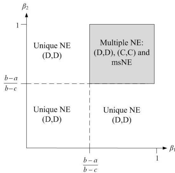
Figure 1. Equilibria in the simultaneous game under complete information.
