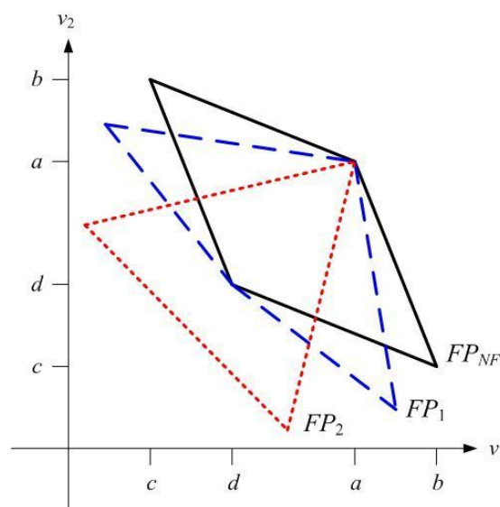
Figure 4. Set of feasible payoffs for \beta_i > 0 .
