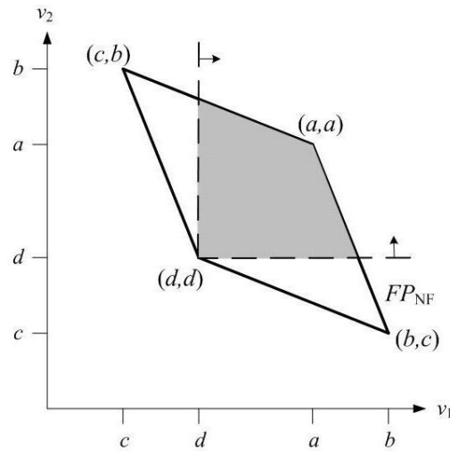
3(b). Individually rational payoffs.
