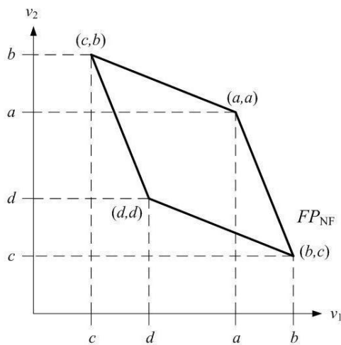
Figure 3. 3(a). Set of feasible payoffs.
