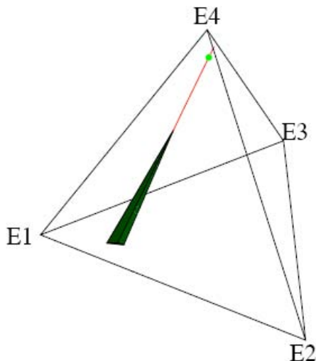
Figure 2. The set V_0 is shown by the green pyramid. The red orbit connects \hat{\mathbf{x}} , the top of the pyramid, the Nash equilibrium N_{1234} and the target point N_{234} for the line segment spanned s by \hat{\mathbf{x}} and N_{1234} .
