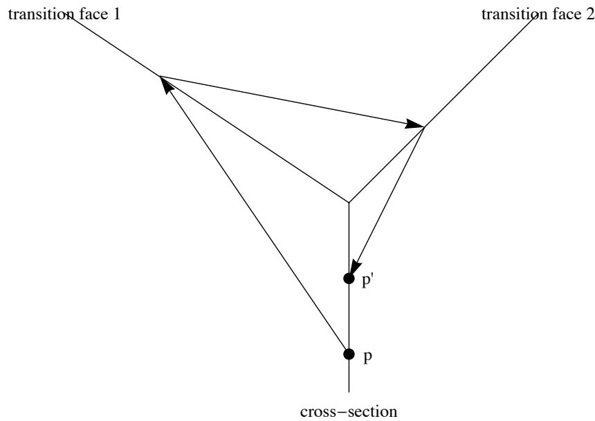
Figure 3. A simplified drawing of the kind of return map we will use below.
