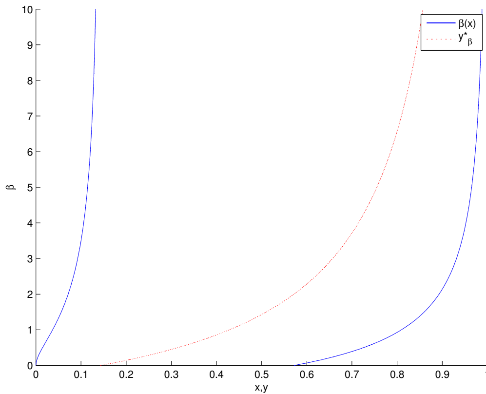
Figure 1. Newman’s solution.
