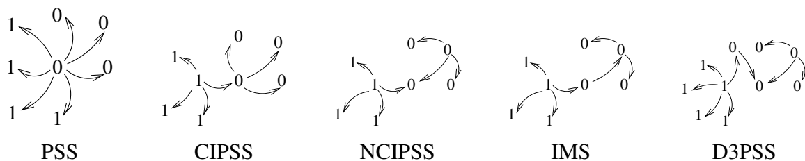
Figure 1. Networks architectures.
