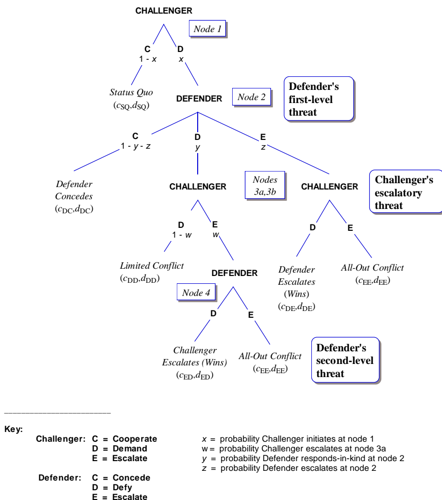
Figure 7. The Asymmetric Escalation Game (Zagare and Kilgour, [33]).
