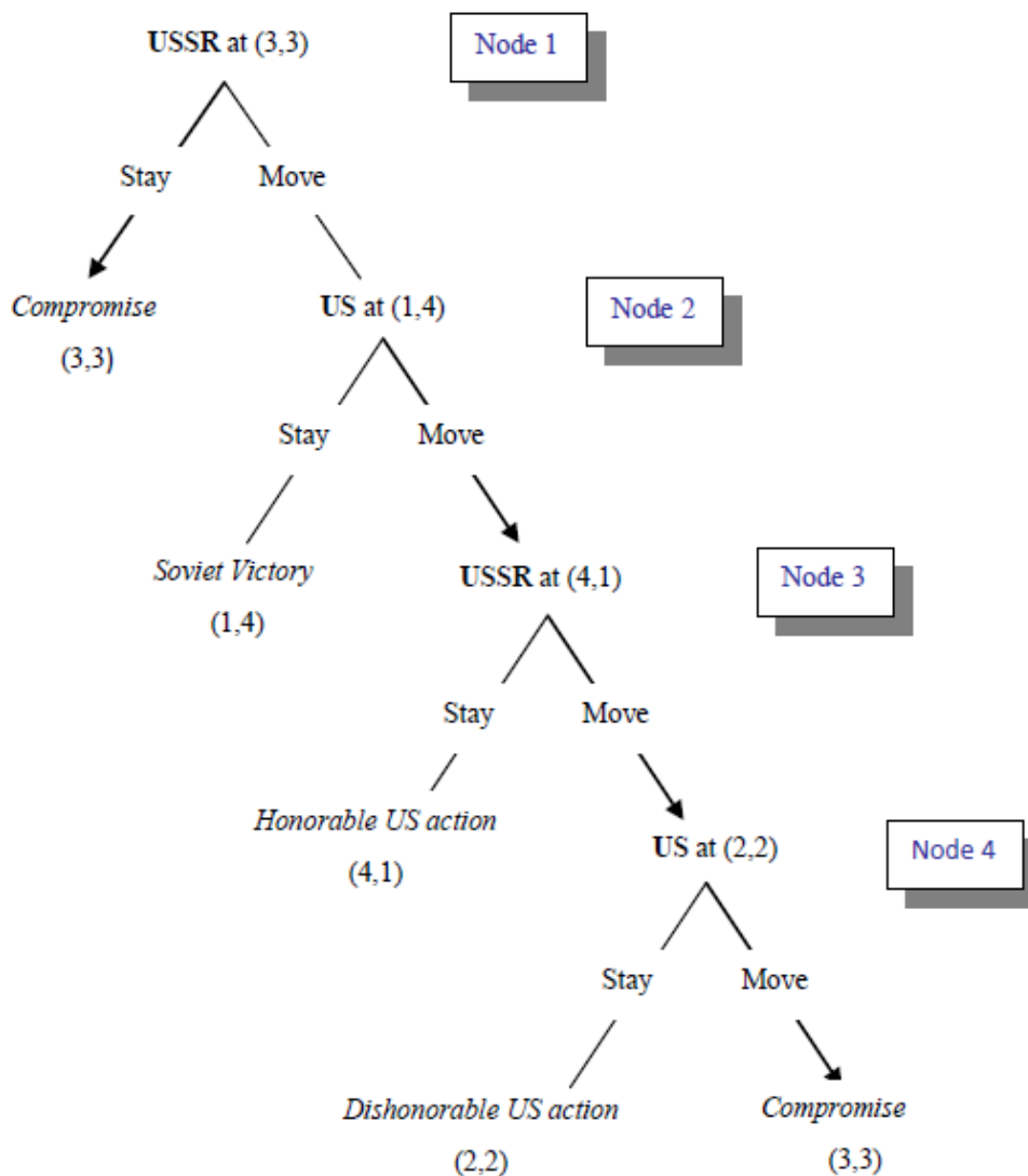
Figure 5. Moves and Countermoves during the Cuban Missile Crisis, starting with the Soviet Union at the Compromise Outcome (3,3).
