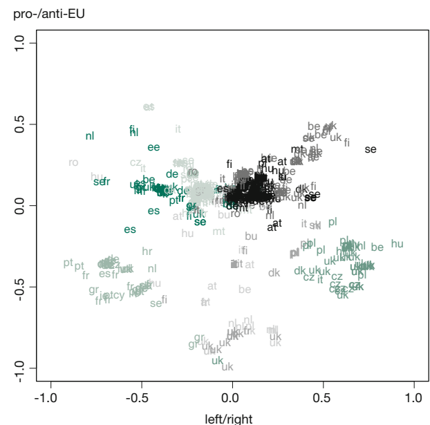
Figure 1 Voting model
