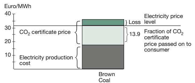
Figure 2 Variable Cost of Brown Coal-Based Electricity Production Including CO 2 Prices Under a Complete Auctioning Regime
