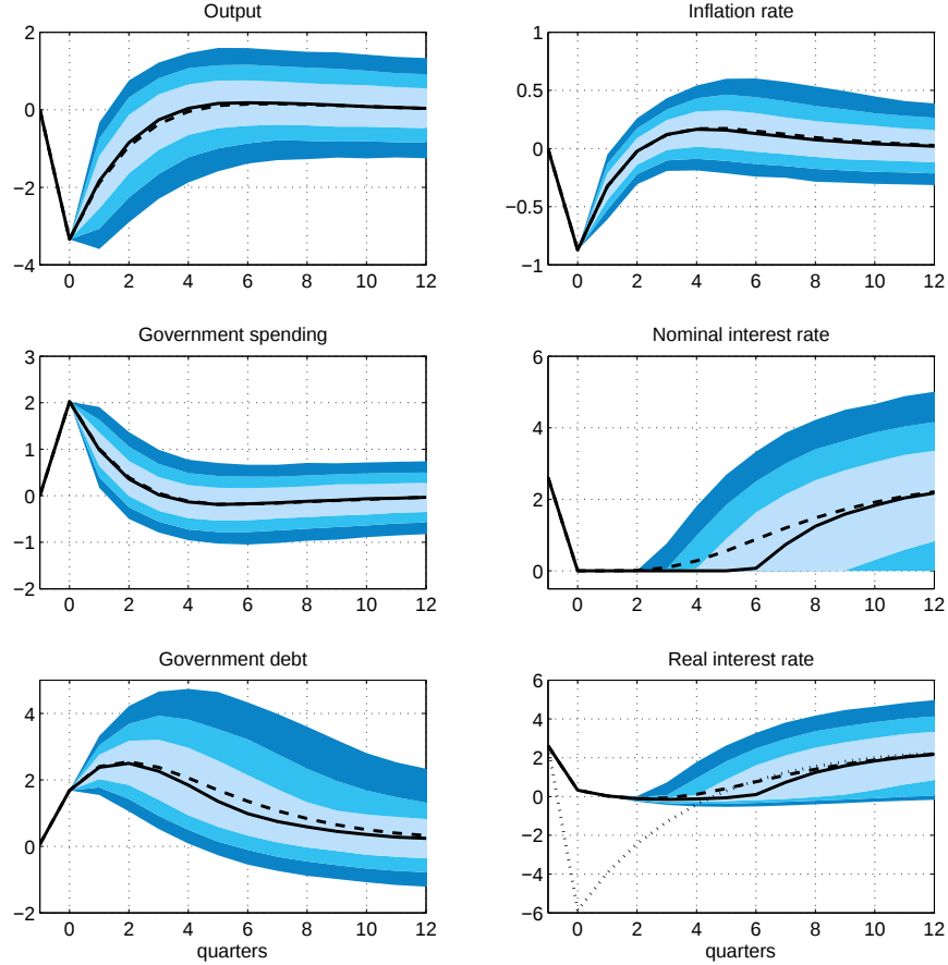
Figure 1: Impulse responses to a negative demand shock
