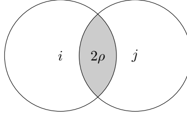
Figure 1: Student demand for i and j overlap by a factor of 2\rho .
