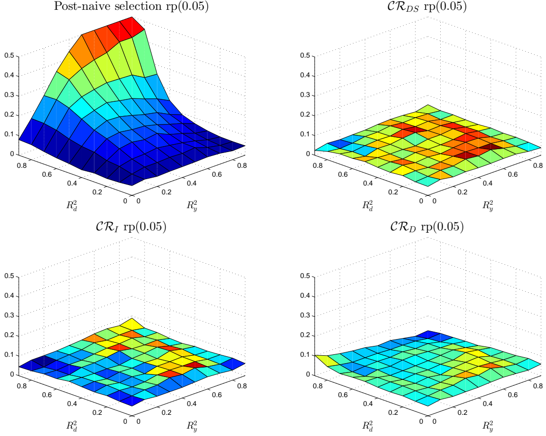
FIGURE 3. The figures display the \text{rp}(0.05) of the confidence region based on post-naive selection and the proposed confidence regions based on optimal instrument ( \mathcal{CR}_D and \mathcal{CR}_I ) and double selection ( \mathcal{CR}_{DS} ). There are a total of 100 different designs with \alpha_0 = 0.25 . The results are based on 1000 replications for each design.
