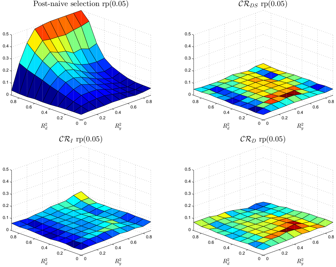
FIGURE 2. The figures display the rp(0.05) of the confidence region based on post-naive selection and the proposed confidence regions based on optimal instrument ( \mathcal{CR}_D and \mathcal{CR}_I ) and double selection ( \mathcal{CR}_{DS} ). There are a total of 100 different designs with \alpha_0 = 0 . The results are based on 1000 replications for each design.
