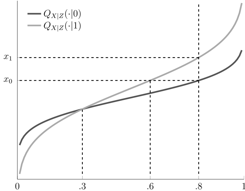
Figure 1: Consider the simple CRC model (1), Y = B_0 + B_1X , and suppose Z is binary. Conditional on R = 0.8 , X assumes two values ( x_0 and x_1 ) depending on the realization of Z . Since Z \perp\!\!\!\perp B \mid \{R = 0.8\} , a mean regression of Y on X conditional on R = 0.8 identifies the means of the intercept and slope coefficients, \mathbb{E}(B_0 \mid R = 0.8) and \mathbb{E}(B_1 \mid R = 0.8) . For the plotted quantile functions, the relevance condition I5 holds for almost every r \in (0, 1) , since the curves intersect at only one point. Hence the previous argument yields \mathbb{E}(B \mid R = r) for all r \in (0, 1) and averaging then gives \mathbb{E}(B) . Note also that the instrument's effect is nonmonotonic—it is positive for units with large R (above R = 0.3 ) and negative for units with small R .
