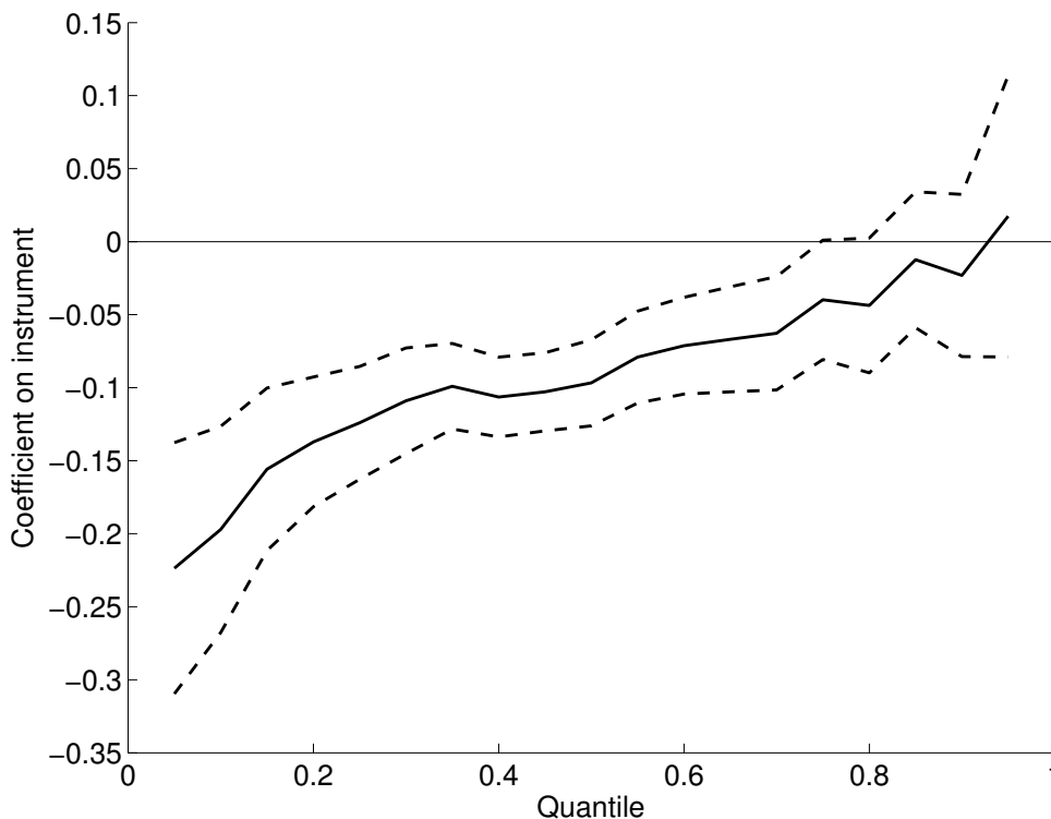
Figure 2: Plot of estimation results from several linear quantile regressions of treatment X (change in TSP, where TSP here is in units of 1 \times 10^{-4} grams/ \text{m}^3 rather than 1 \times 10^{-6} grams/ \text{m}^3 = \mu\text{g}/\text{m}^3 ) on the instrument Z_2 (nonattainment status) and controls. The solid line plots the estimated coefficient on the instrument on the vertical axis against the corresponding quantile on the horizontal axis, from .05 to .95 in .05 increments. The dotted lines plot simultaneous confidence intervals for each of these quantiles.
