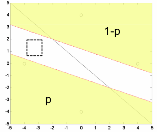
Figure 3: Voronoi Tessellations for Candidates C'_1, C'_2
