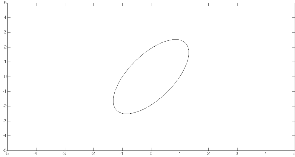
Figure 8: Indifference Curve for d^W(\mathbf{0}, C) = 1 .
