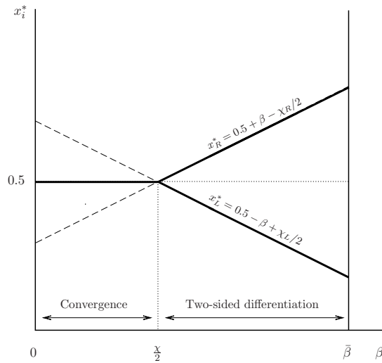
Figure 1: Symmetric case: \chi_L = \chi_R \equiv \chi .
