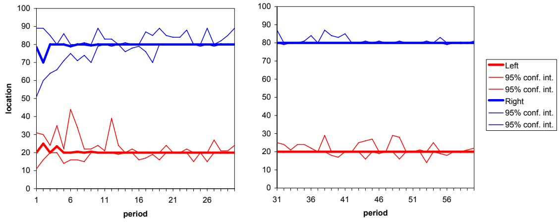
(e) Treatment 5: x_L^* = 20 & x_R^* = 80 .
