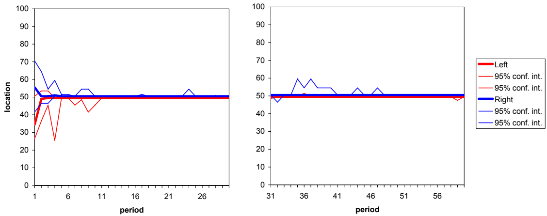
(c) Treatment 3: x_L^* = x_R^* = 50 .
