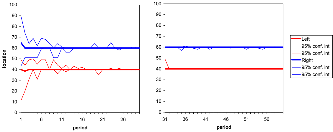
(b) Treatment 2: x_L^* = 40 & x_R^* = 60 .
