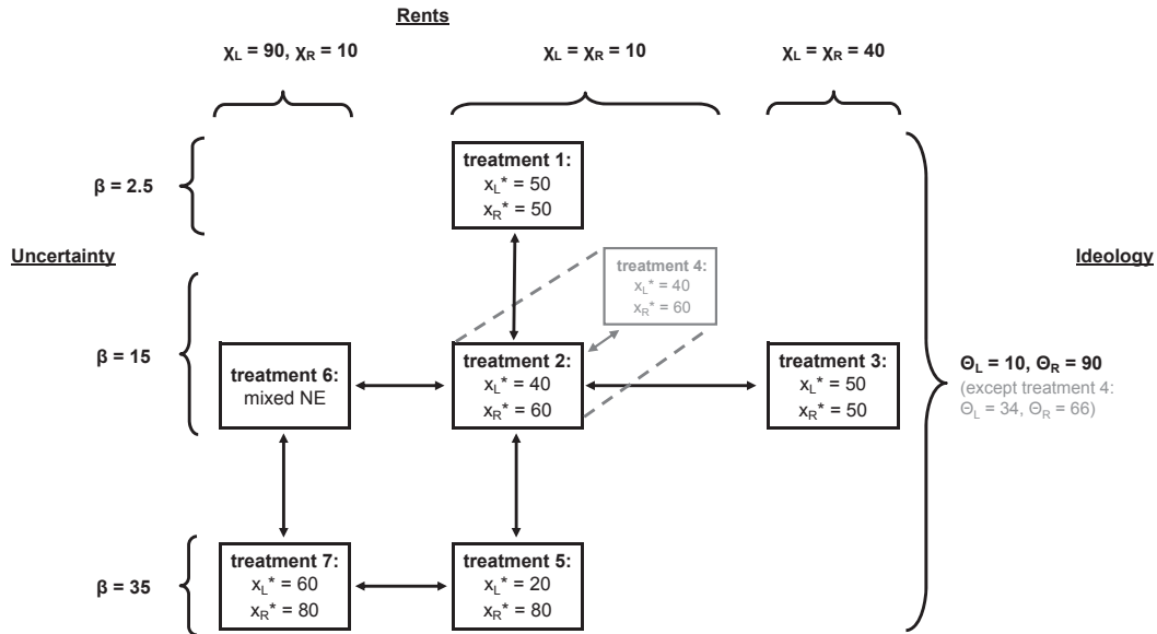
Figure 6: Overview of the comparisons between Treatments.
