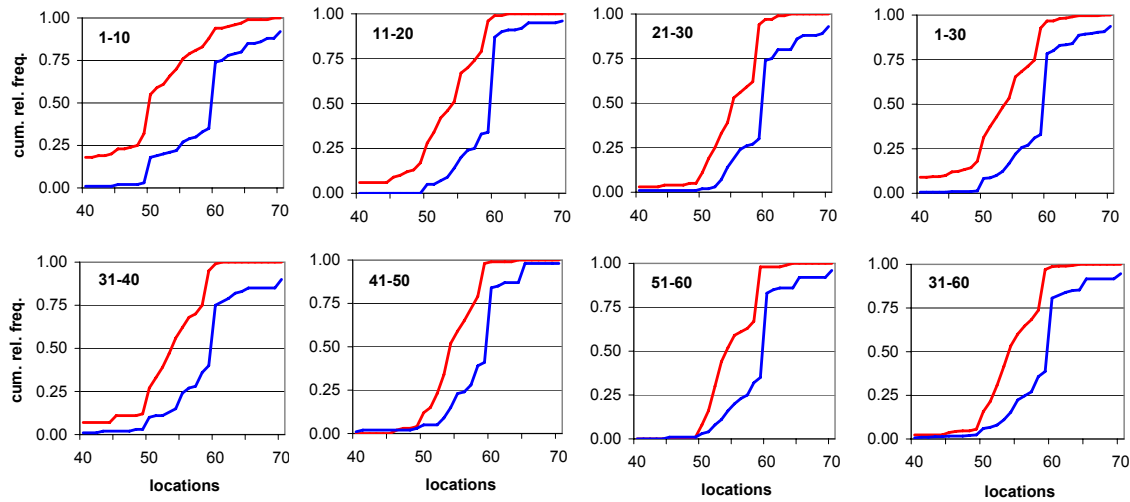
(e) Cumulative relative frequencies in different subintervals.
