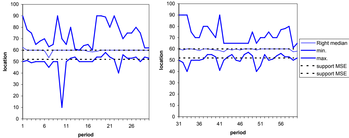
(b) Median, minimum and maximum locations of the Right players.
