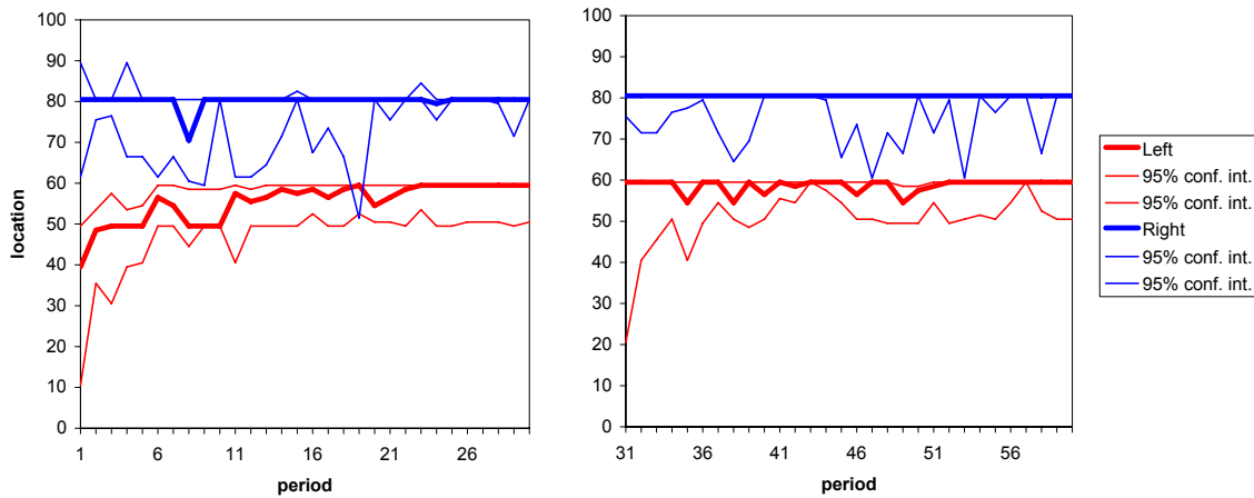
(f) Treatment 7: x_L^* = 60 & x_R^* = 80 .
