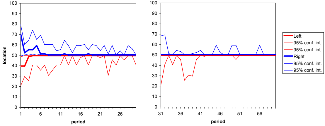
(a) Treatment 1: x_L^* = x_R^* = 50 .
