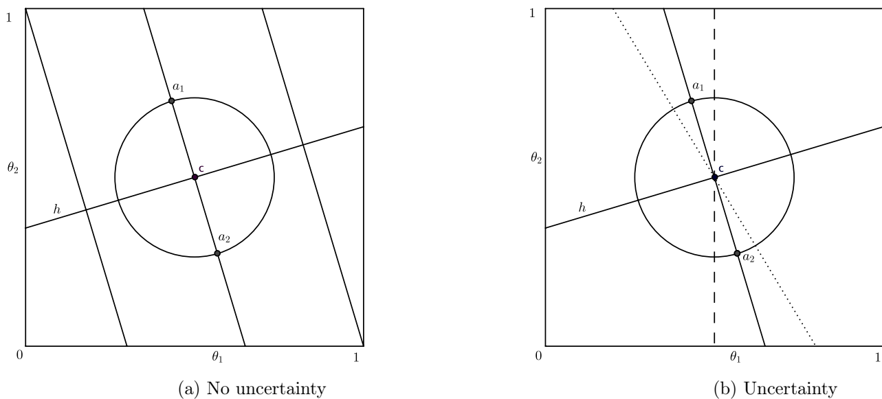
Figure 1: Uncertainty vs. no uncertainty in the linear case
