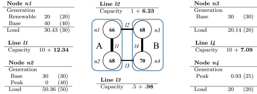
Figure 1: Benchmark cases in the illustrative two-zone, four-node network; generation capacity and reference load in brackets; investment in bold; nodal prices given in the circles in the figure
