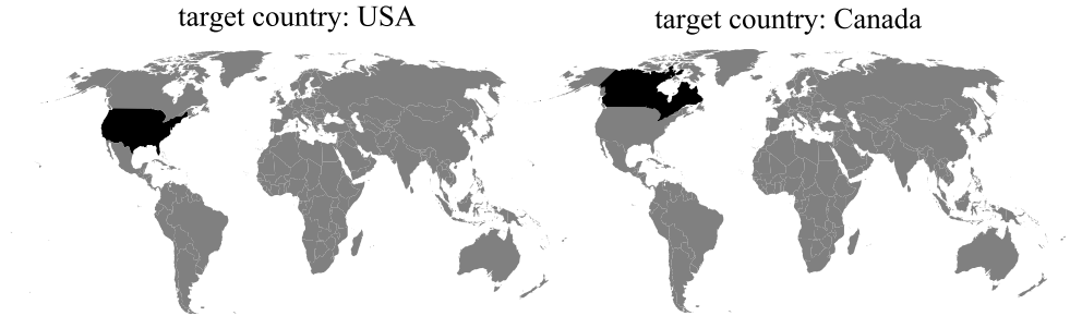
Figure 4: Dividing the world in a target country and the rest-of-the-world in the bi-regional model using USA and Canada as examples.
