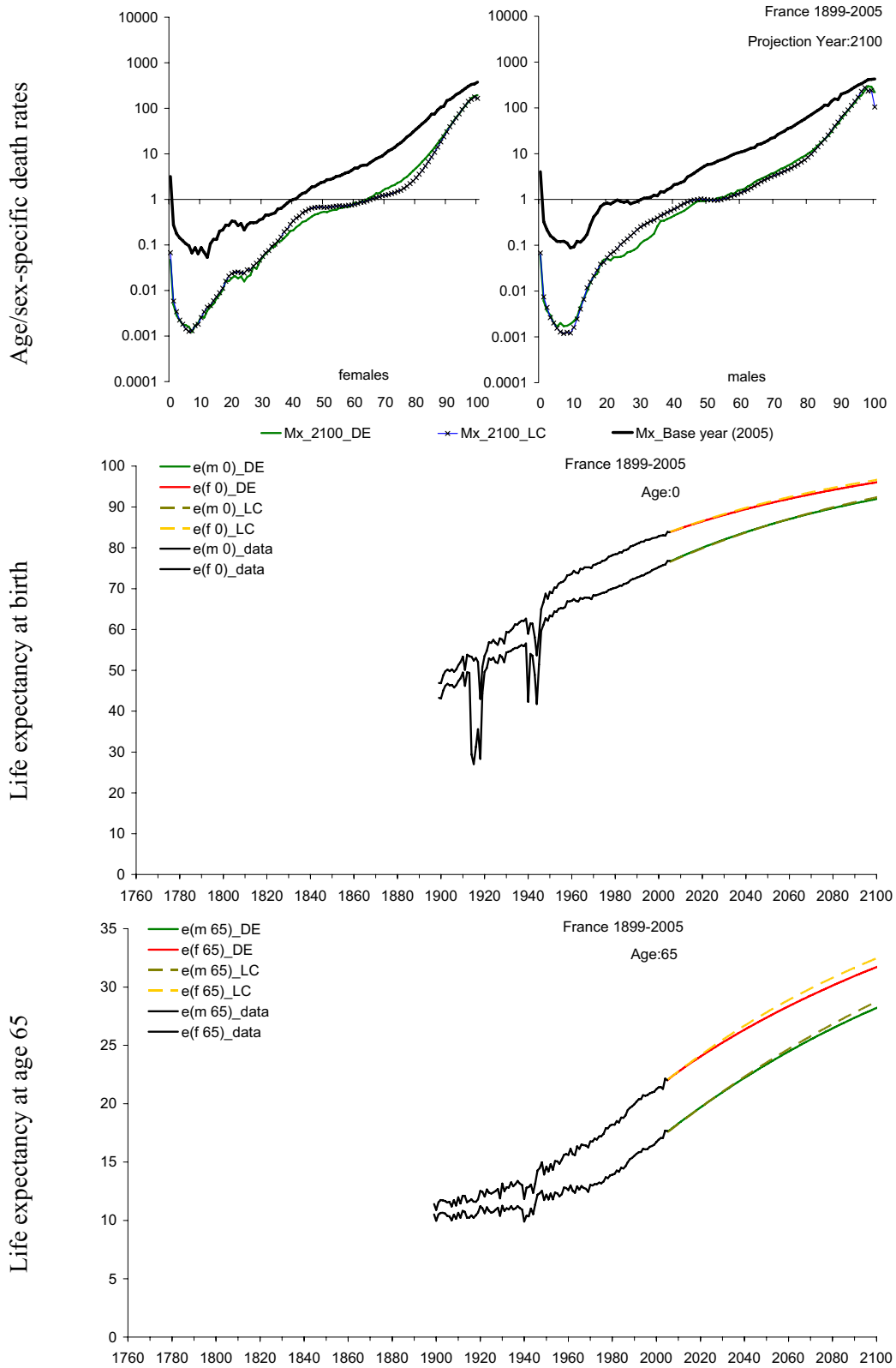
Figure 15. Projected age/sex-specific death rates (per 1000, logarithmic scale) and life expectancies at ages 0 and 65 based on the most recent optimal data periods. France.
