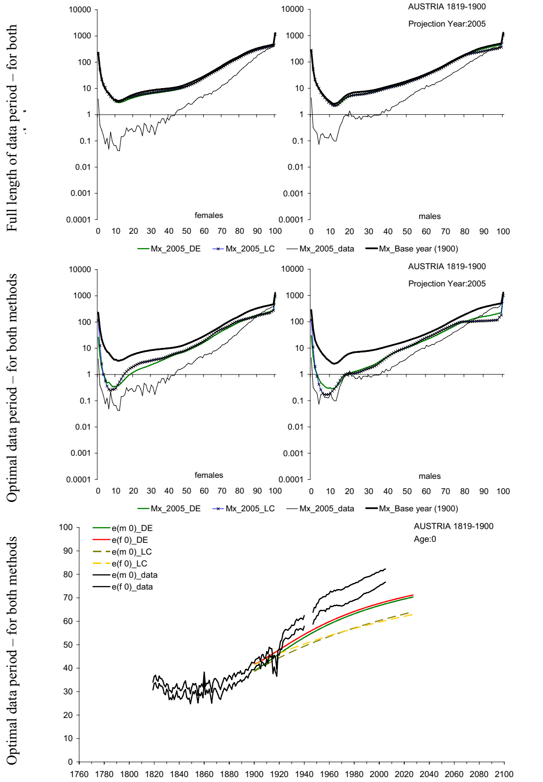
Figure 8. Projected age/sex-specific death rates (per 1000, logarithmic scale) and life expectancy at birth since 1900 based on data prior to 1900. Austria.
