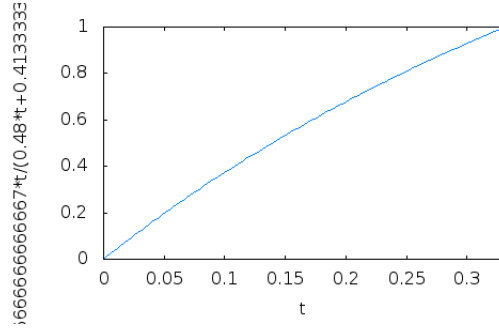
Figure 1: Army size as a function of the tax-rate
