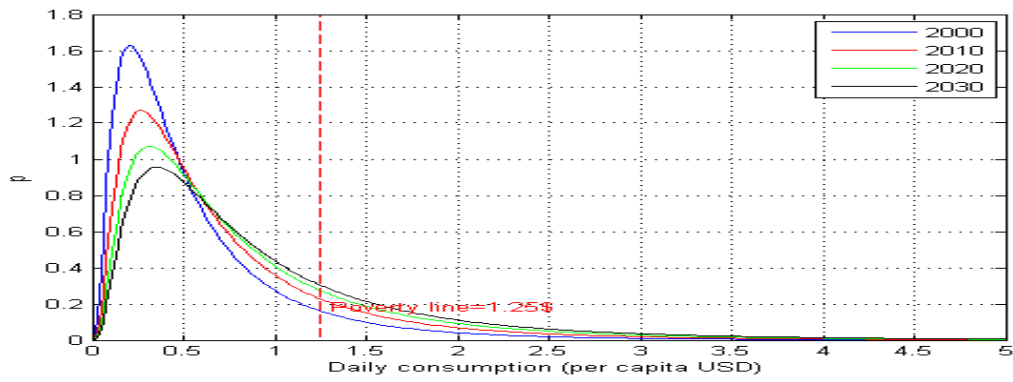
Figure 5f. Tanzania: Probability density functions, various years
