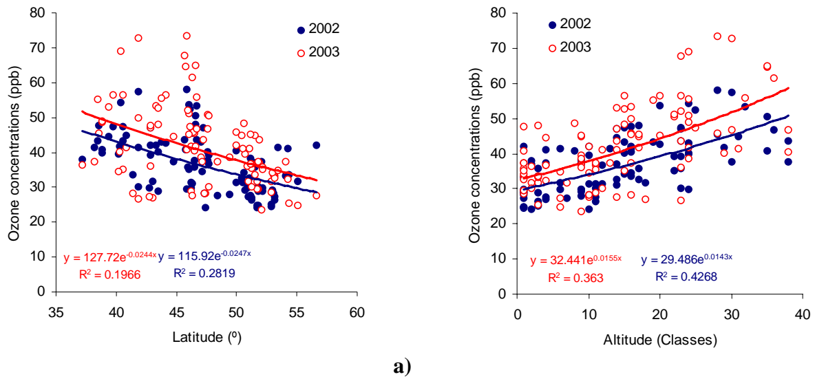
Figure 3.5.3-4: Regression analysis for ozone concentrations (ppb) of Level II plots versus latitude (a) and (b) altitude respectively for the years 2002 and 2003.
