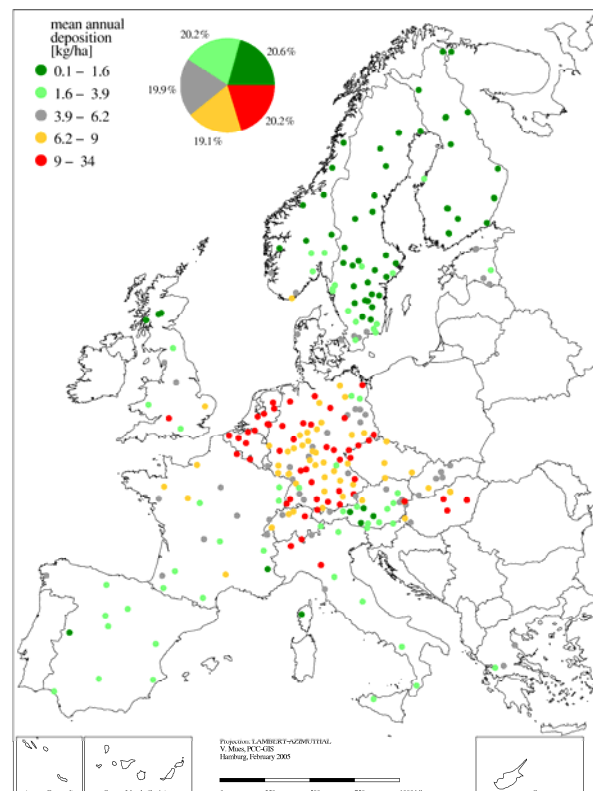
Figure 3.2.3.1-6: Mean annual ammonium ( \text{N-NH}_4 ) throughfall deposition 1999 to 2001.
