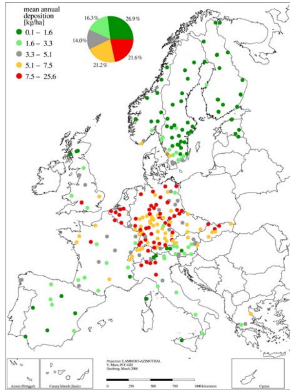
Figure 3.2.3-7: Mean annual ammonium (N- NH 4 + ) throughfall deposition 2001 to 2003.
