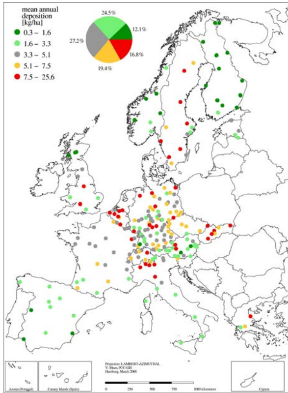
Figure 3.2.3-6: Mean annual ammonium (N- NH 4 + ) bulk deposition 2001 to 2003.
