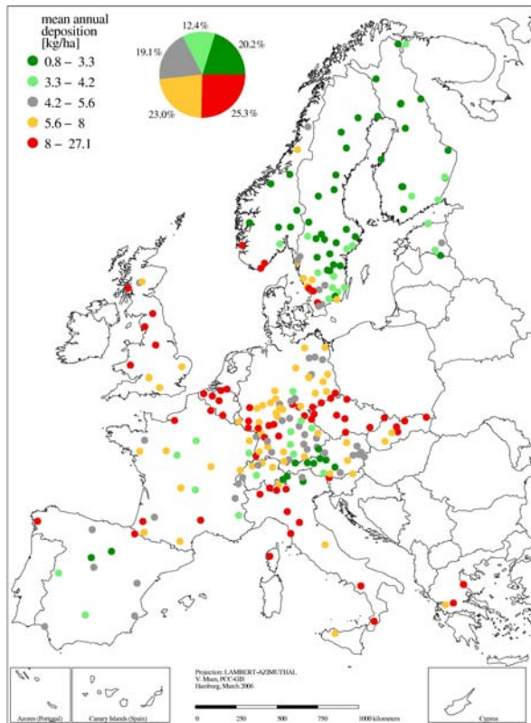
Figure 3.2.3-3: Mean annual sulphate (S- \text{SO}_4^{2-} ) throughfall deposition 2001 to 2003.
