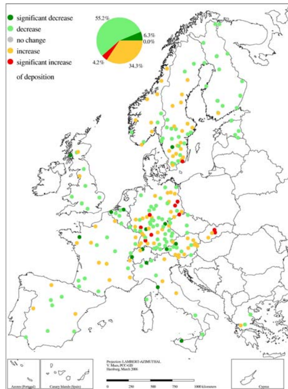
Figure 3.2.3-11: Trends of ammonium (N-NH 4 + ) in throughfall deposition 1998 to 2003.
