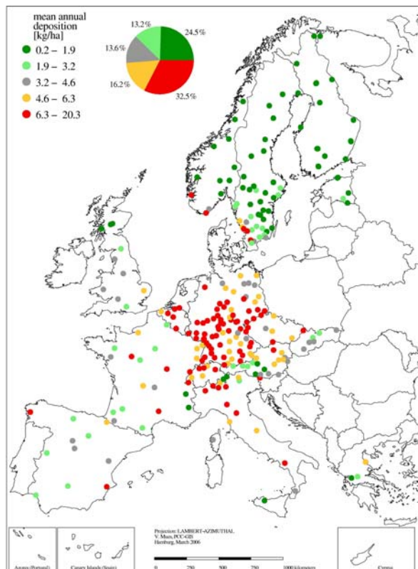
Figure 3.2.3-5: Mean annual nitrate (N- \text{NO}_3^- ) throughfall deposition 2001 to 2003.
