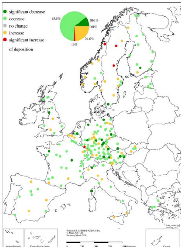
Figure 3.2.3-12: Trends of ammonium (N-NH 4 + ) in bulk deposition 1998 to 2003.
