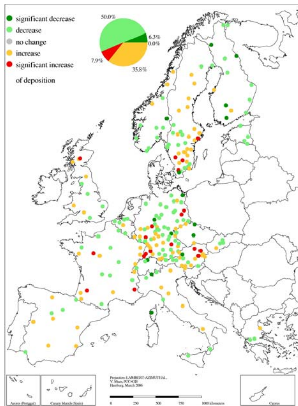
Figure 3.2.3-10: Trends of nitrate (N-NO 3 - ) in throughfall deposition 1998 to 2003.
