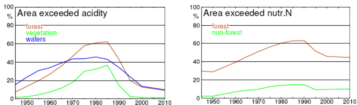
Figure 3.4.1-2: Ecosystem area exceeded by acidity (left) and nutrient nitrogen (right).
