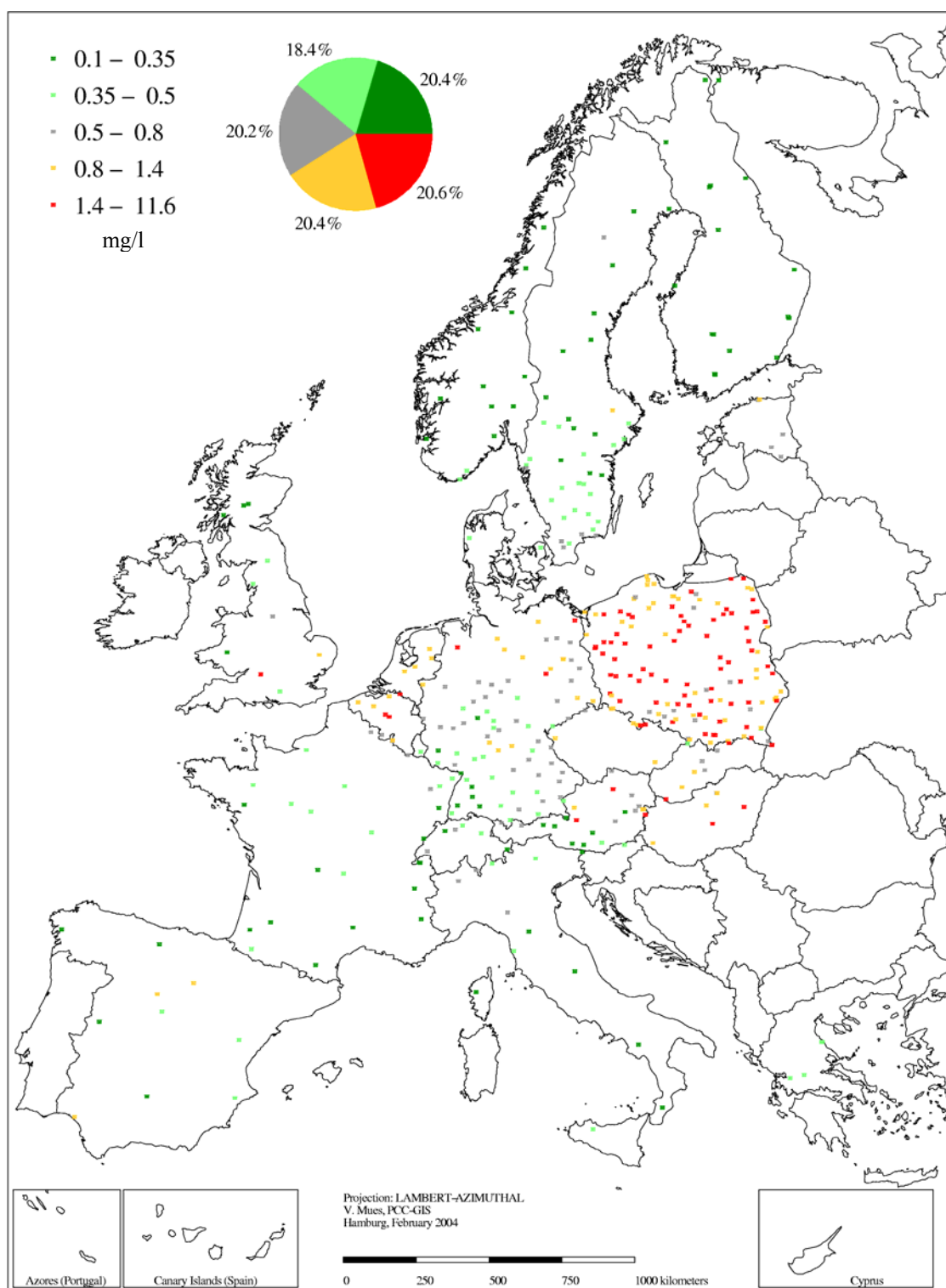
Figure 3.2.3.2-1: Geographic variation of the volume weighted mean \text{N-NH}_4 concentration in mg/l between 1999 and 2001 at 407 Level II plots.
