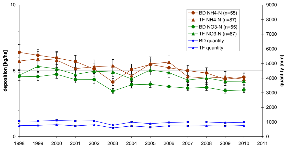
Figure 4.4.2-4: Trend of nitrate ( \text{NO}_3\text{-N} ) and ammonia ( \text{NH}_4^+\text{-N} ) bulk and throughfall deposition and precipitation volume (quantity) of plots with continuous measurements from 1998 to 2010. Error bars show the standard error of the mean.
