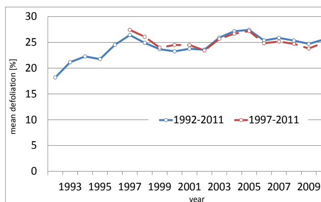
Figure 3.1.3.6-1: Mean defoliation in two periods (1992-2011 and 1997-2011)
