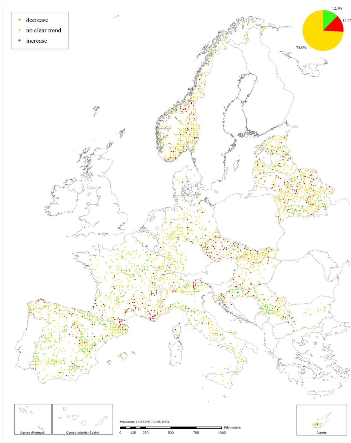
Figure 3.1.3.1-3: Development of mean plot defoliation (slope of linear regression) of all species over the years 2002 – 2011.
