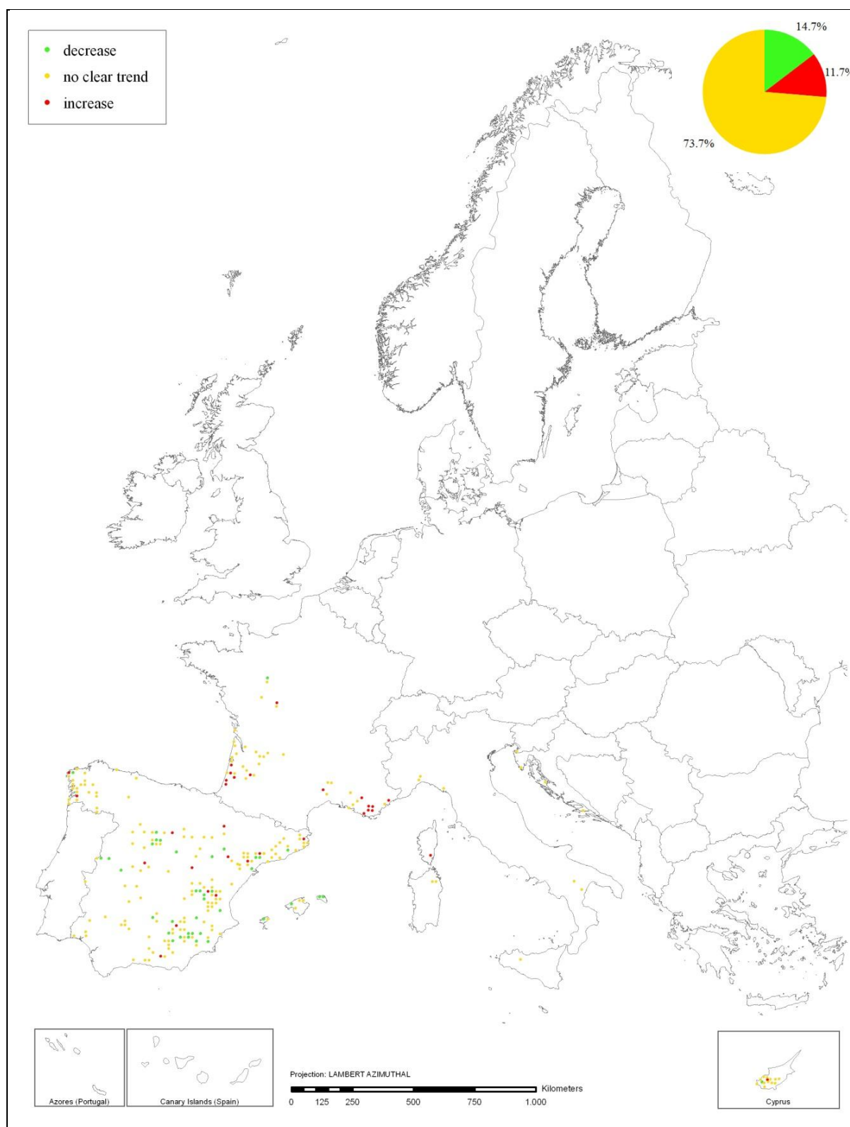
Figure 3.1.3.4-3: Development of mean plot defoliation (slope of linear regression) of Mediterranean lowland pines over the years 2002-2011
