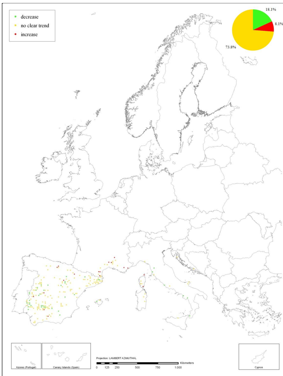
Figure 3.1.3.8-3: Development of mean plot defoliation (slope of linear regression) of evergreen oak species over the years 2002-2011
