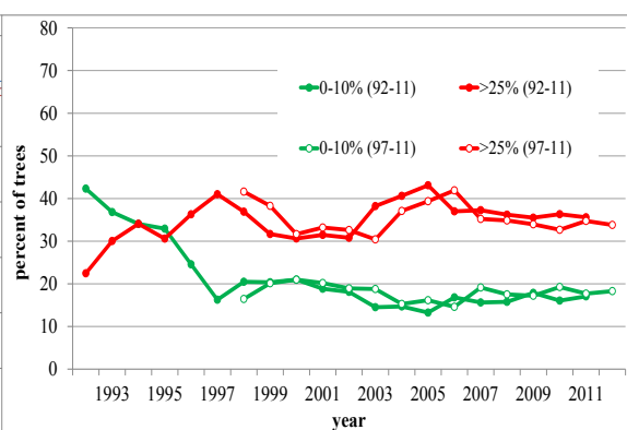
Figure 3.1.3.6-2: Shares of trees of defoliation 0-10% and > 25% in two periods (1992-2011 and 1997-2011)
