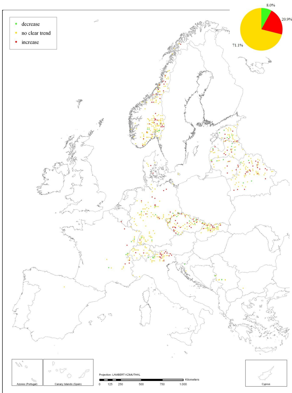
Figure 3.1.3.3-3: Development of mean plot defoliation (slope of linear regression) of Picea abies over the years 2002-2011
