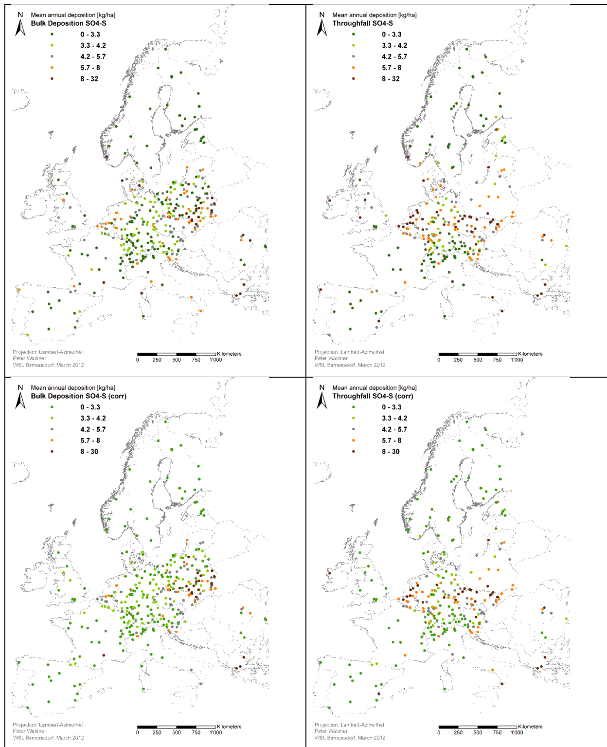
Figure 4.4.1-1 Mean annual sulphate sulphur ( \text{SO}_4^- ) throughfall and bulk deposition 2008 to 2010 with and without sea salt deposition included. Corr = no sea salt included
