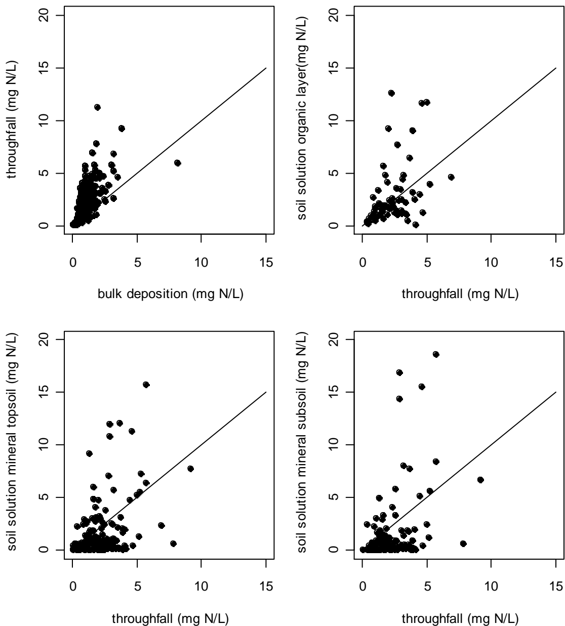
Figure 5.3-1: Concentration of dissolved inorganic nitrogen (NH 4 + + NO 3 - ) in bulk precipitation, throughfall precipitation, and soil solution (top right: organic layer, bottom left: mineral topsoil 0-40 cm and bottom right: mineral subsoil 40-80 cm) on selected ICP-Forests level II plots.
