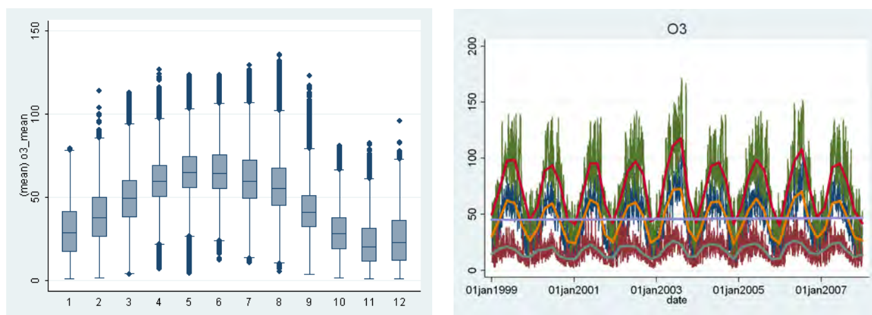
Figure 14: Ozone ( O_3 ) Variation Across Counties and Over Time
