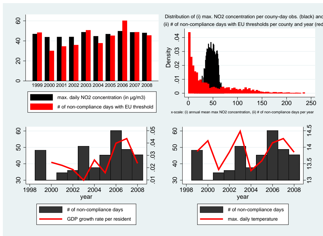
Figure 13: Distribution of Nitrogen Dioxide ( NO_2 ) Concentration and Non-Compliance Days: Identifying Variation
