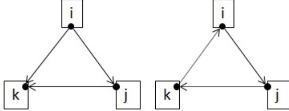
Figure 1: The left triadic structure corresponds to the transitive triplets effect CC^1 . The right triadic structure illustrates the 3-cycles effect CC^2 and is non-hierarchical, since all nodes have the same roles as lenders and borrowers.
