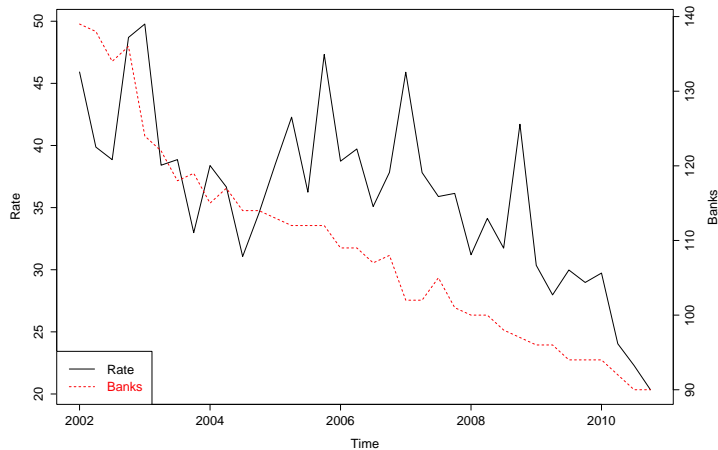
Figure 2: The evolution of the basic rate parameter and the number of banks (dashed) from 2002Q1 to 2010Q4.
