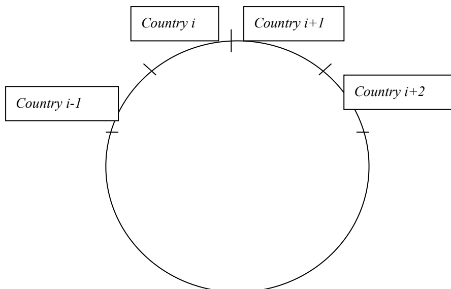
Figure 1. Salop model
