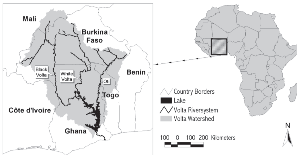
Figure 1: Volta basin
