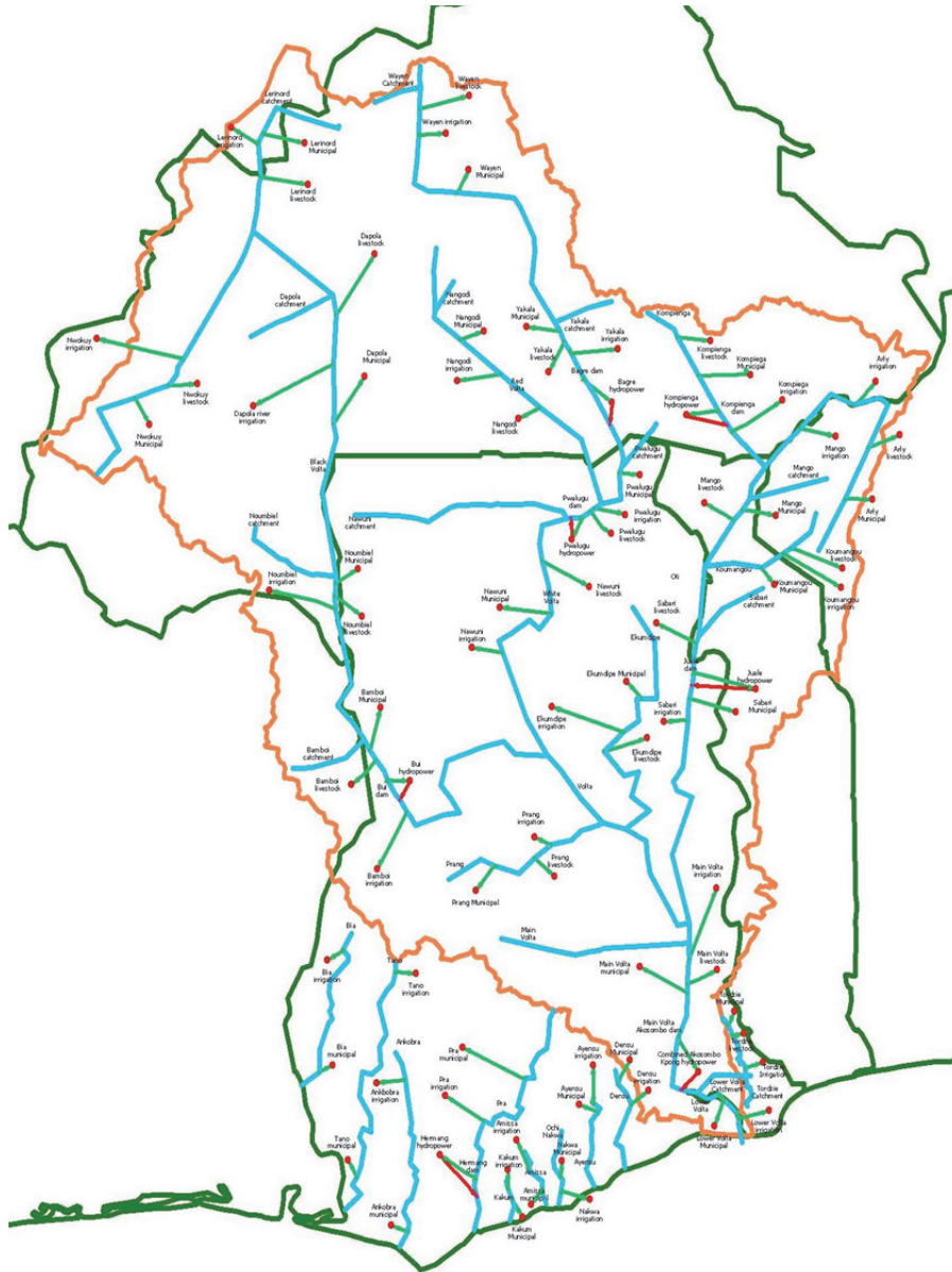
Figure 5: WEAP Schematic for the entire Volta basin and the southwestern and coastal basins of Ghana
