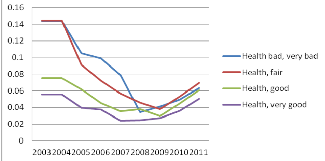
Fig 4: FGT, \alpha=1
