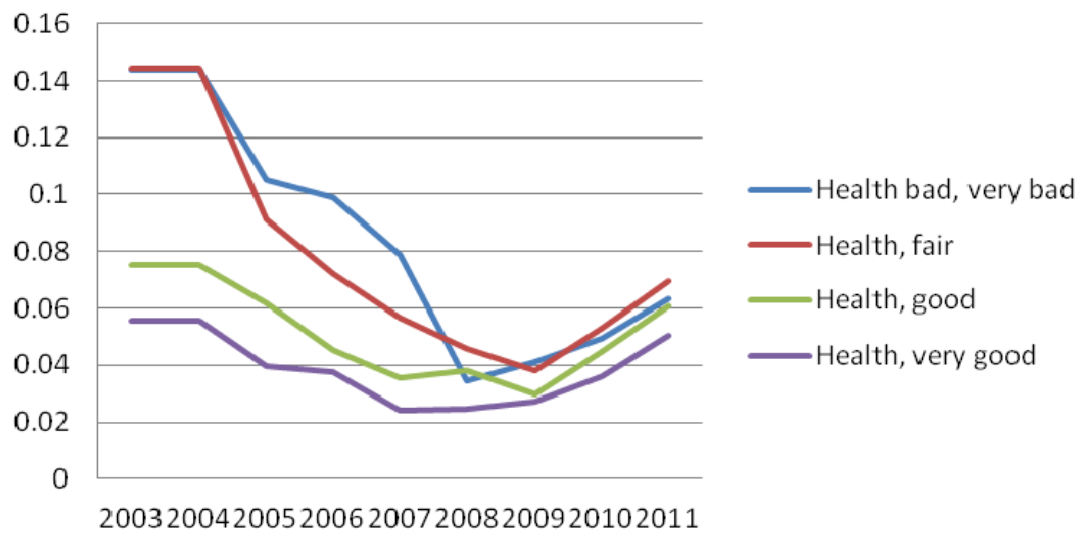
Fig 4: FGT, \alpha=1
