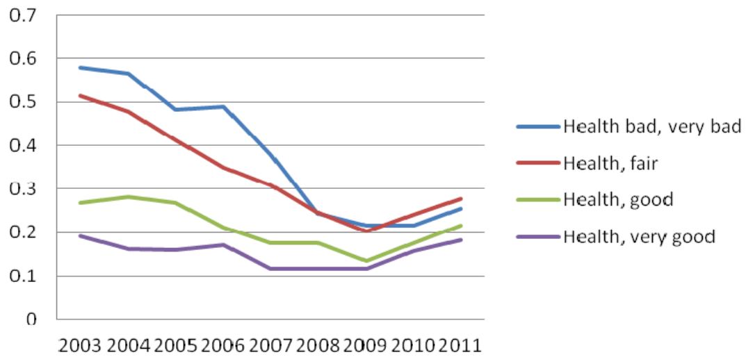
Fig 3: FGT, \alpha=0
