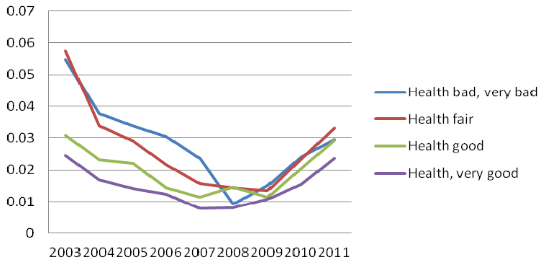
Fig 5: FGT, \alpha=2
