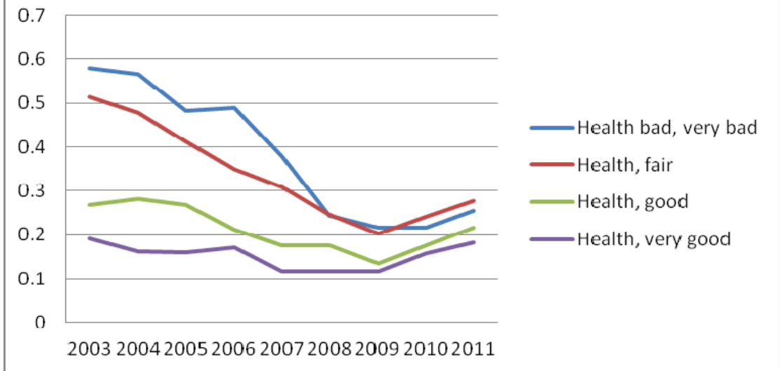
Fig 3: FGT, \alpha=0
