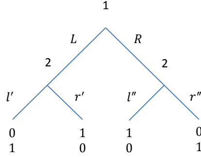
Figure 2. An extensive-form game with perfect information that is not BI -acyclic. The best-improvement graph of the game has the following closed walk: (L, l'') , (R, l'') , (R, r' r'') , (L, r' r'') and back to (L, l' l'') .
