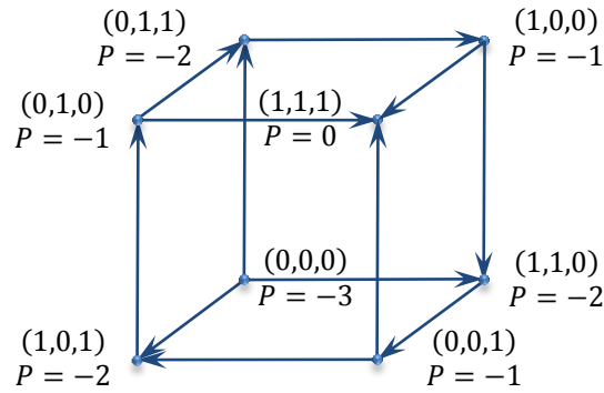
Figure 1. The cube-like improvement (and best-improvement) graph of a finite 2 \times 2 \times 2 game that is (i) weakly acyclic but (ii) not acyclic, (iii) not solvable by iterated elimination of never-best response strategies and (iv) has the property that every subgame (which corresponds to a k -dimensional face of the cube, with 0 \leq k \leq 3 ) has a unique equilibrium. The strategies are right and left for player 1, up and down for player 2, and in and out for player 3. Shown for each strategy profile are the players' payoff vector and the value of a weak potential P defined as in the proof of Theorem 1.
