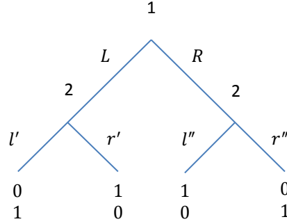
Figure 2. An extensive-form game with perfect information that is not BI -acyclic. The best-improvement graph of the game has the following closed walk: (L, l'') , (R, l'') , (R, r'') , (L, r'') and back to (L, l'') .
