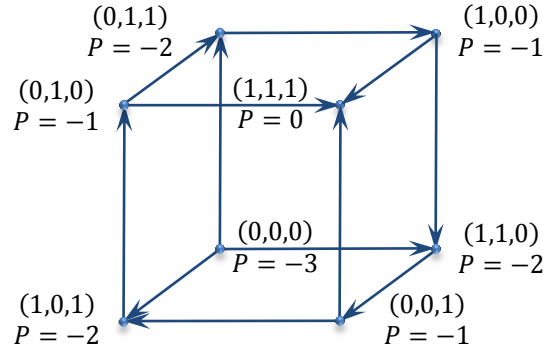
Figure 1. The cube-like improvement (and best-improvement) graph of a finite 2 \times 2 \times 2 game that is (i) weakly acyclic but (ii) not acyclic, (iii) not solvable by iterated elimination of never-best response strategies and (iv) has the property that every subgame (which corresponds to a k -dimensional face of the cube, with 0 \leq k \leq 3 ) has a unique equilibrium. The strategies are right and left for player 1, up and down for player 2, and in and out for player 3. Shown for each strategy profile are the players' payoff vector and the value of a weak potential P defined as in the proof of Theorem 1.
