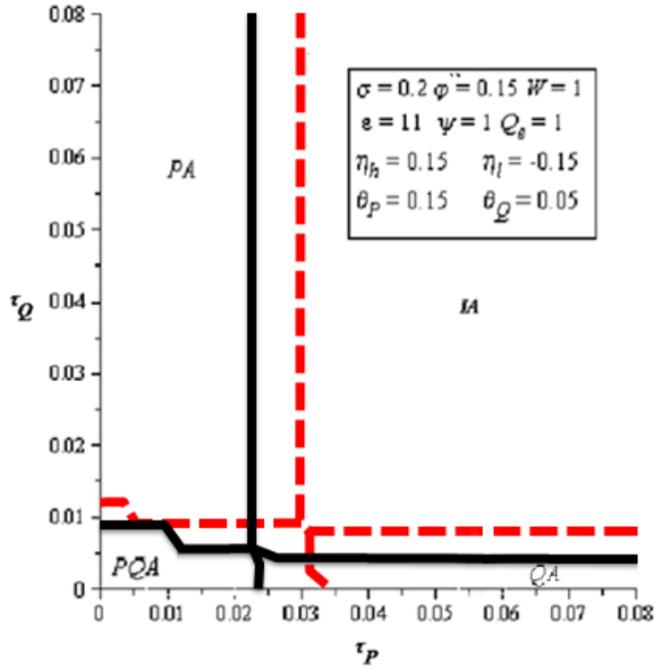
Figure 3. The effect of increasing the elasticity of marginal disutility with respect to labor, \varphi , from 0.1 to 0.15
