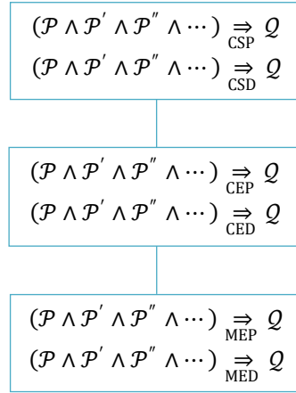
Figure 4. Hesse diagram of the implication relations between attributes of (equilibrium) outcomes in Bayesian games: correlated strategy distributions (CSDs), correlated strategy payoffs (CSPs), correlated equilibrium distributions (CEDs), correlated equilibrium payoffs (CEPs), communication equilibrium distributions (MEDs) and communication equilibrium payoffs (MEPs). A box represents a pair of equivalent implication relations: for all subsets \mathcal{P}, \mathcal{P}', \mathcal{P}'', \dots and Q of (the set of properties of mechanisms) \{S, \tilde{S}, O, \tilde{O}, D, I\} , one implication holds is and only if the other holds. A line represents only one-way implication (between implications): whenever an implication relation in the lower box holds, so does each implication relation in the higher box.
