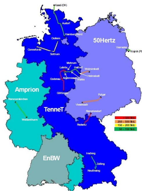
Figure 21: Network elements with more than 50 hours of re-dispatch measures
