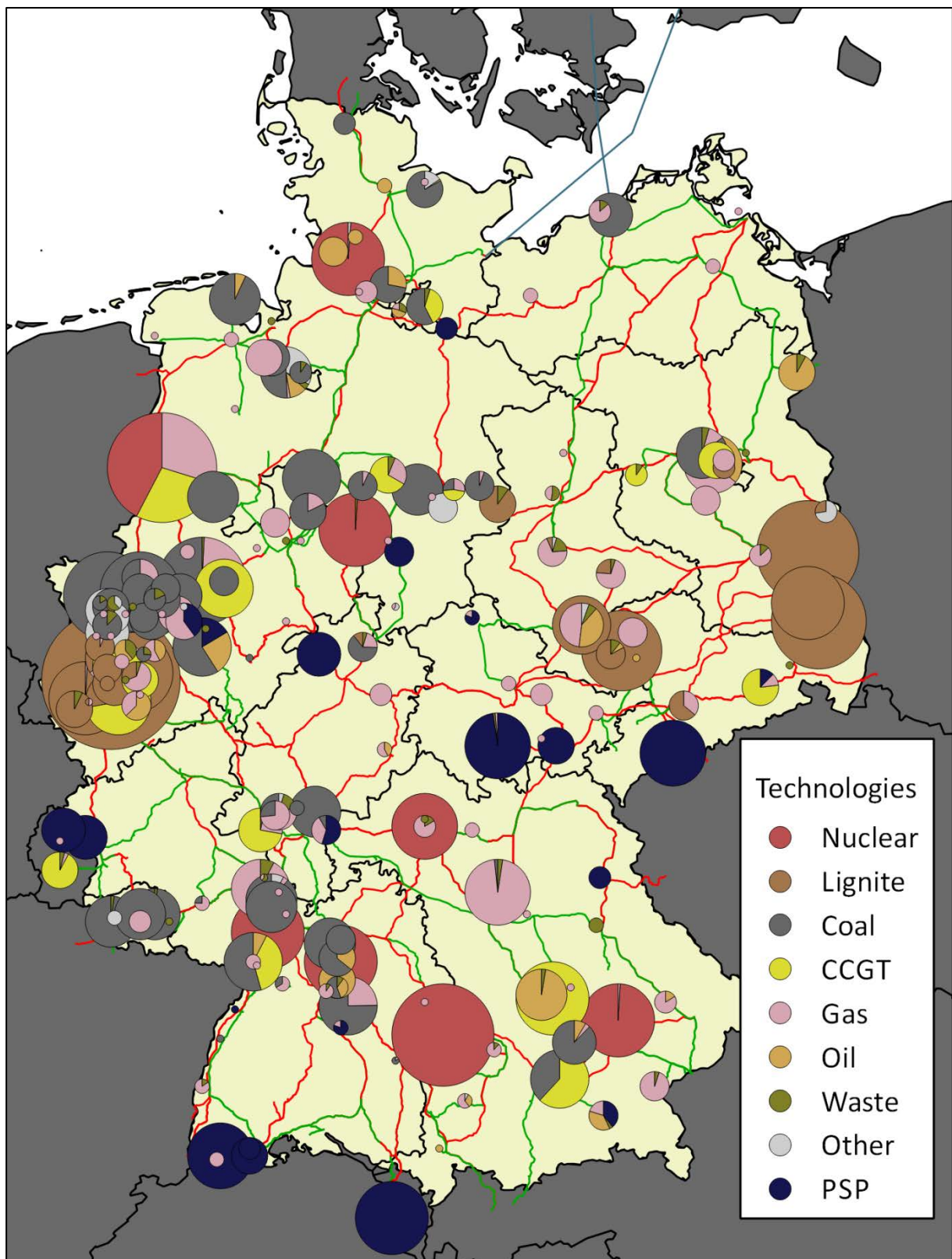
Figure 11: Conventional generation capacity on a nodal level
