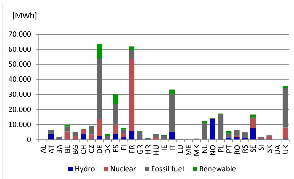
Figure 34: Average generation in 2011 based on ENTSO-E
