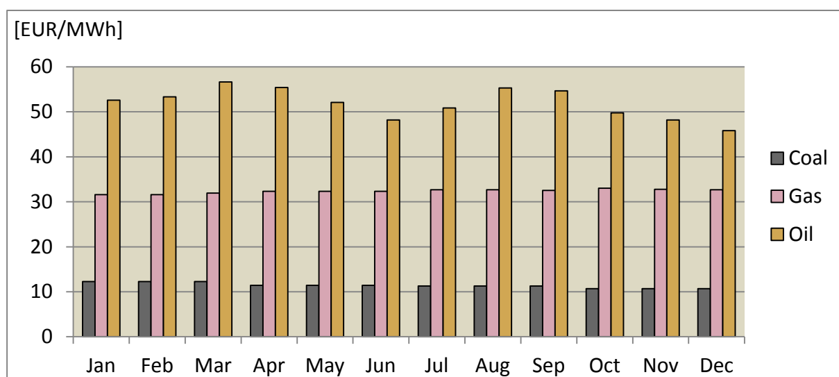
Figure 15: Monthly hard coal, natural gas, and fuel oil prices in 2012
