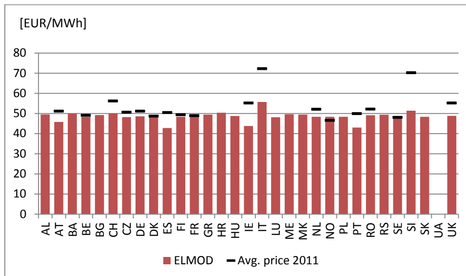
Figure 33: Comparison of modeled prices with historic prices in 2011
