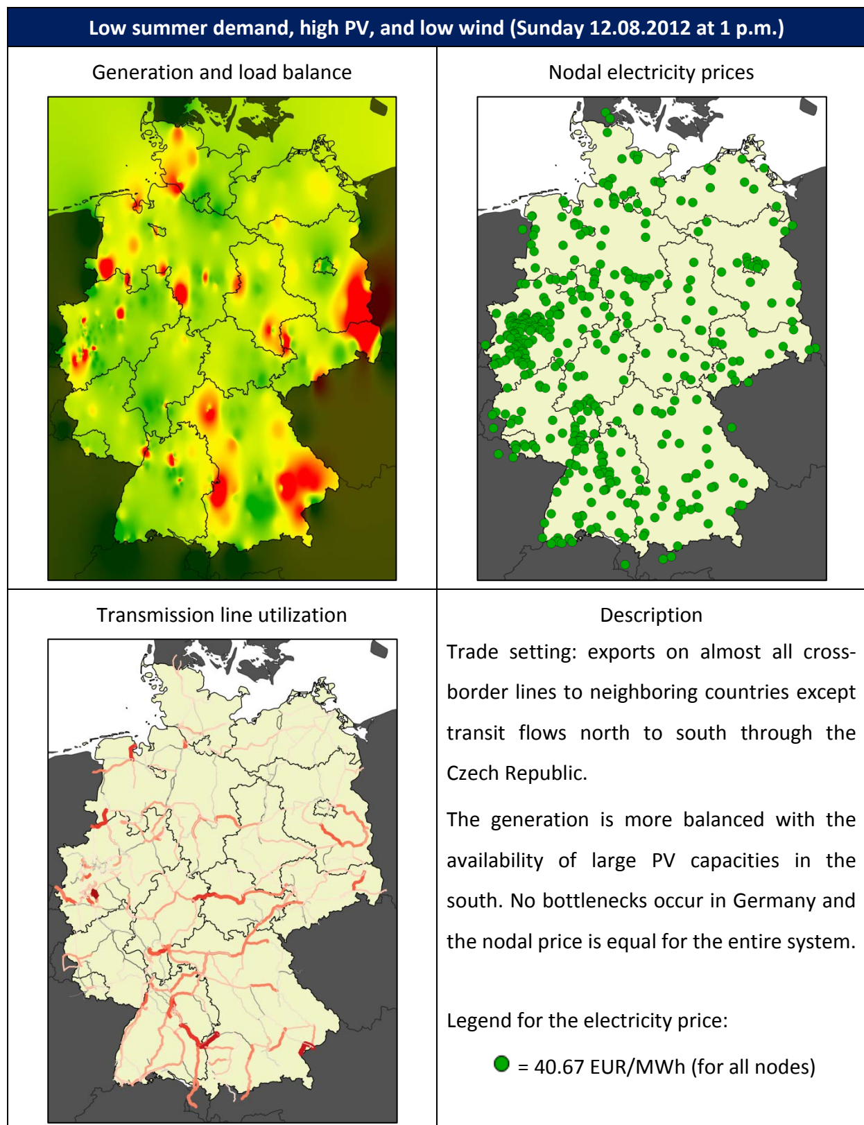
Figure 27: Snap shot of the system with low summer load and very high PV
