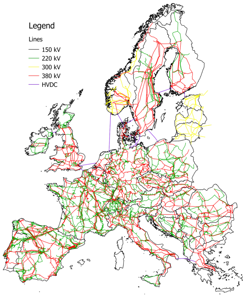
Figure 28: European transmission network
