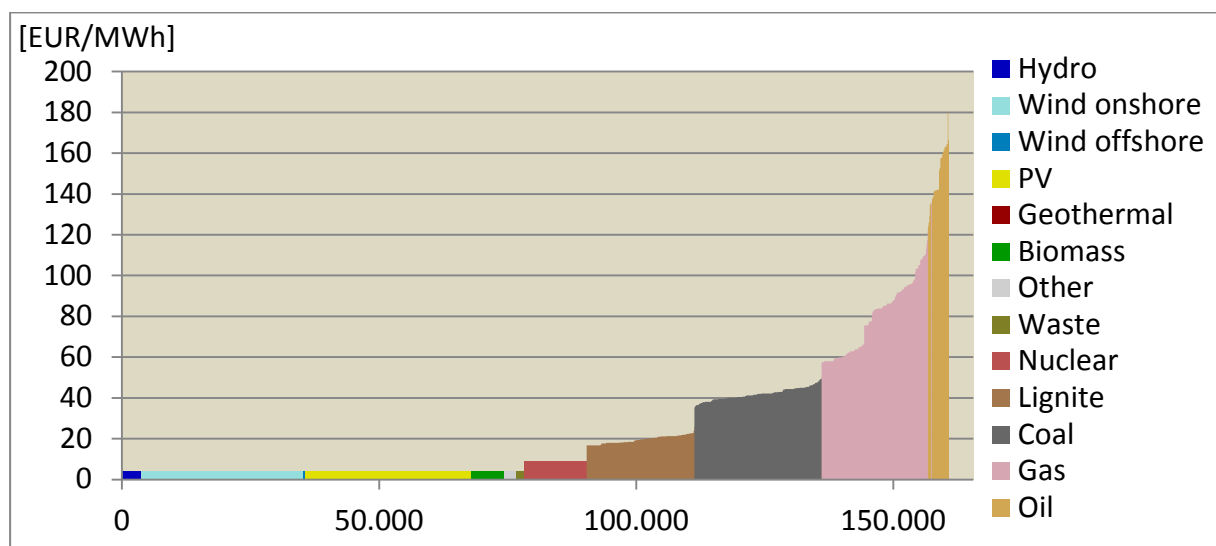
Figure 14: Merit order for the German electricity market with all capacities in 2012
