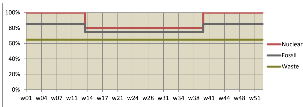
Figure 18: Availability factors for conventional power plants
