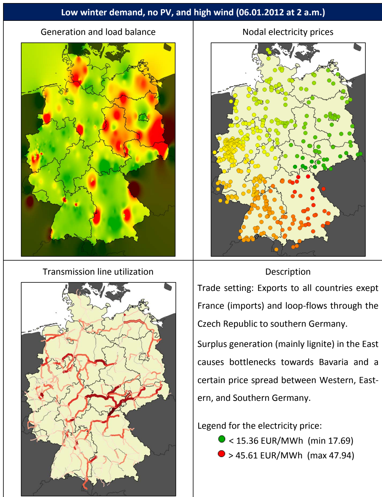
Figure 26: Snap shot of the system with low winter load and high wind generation
