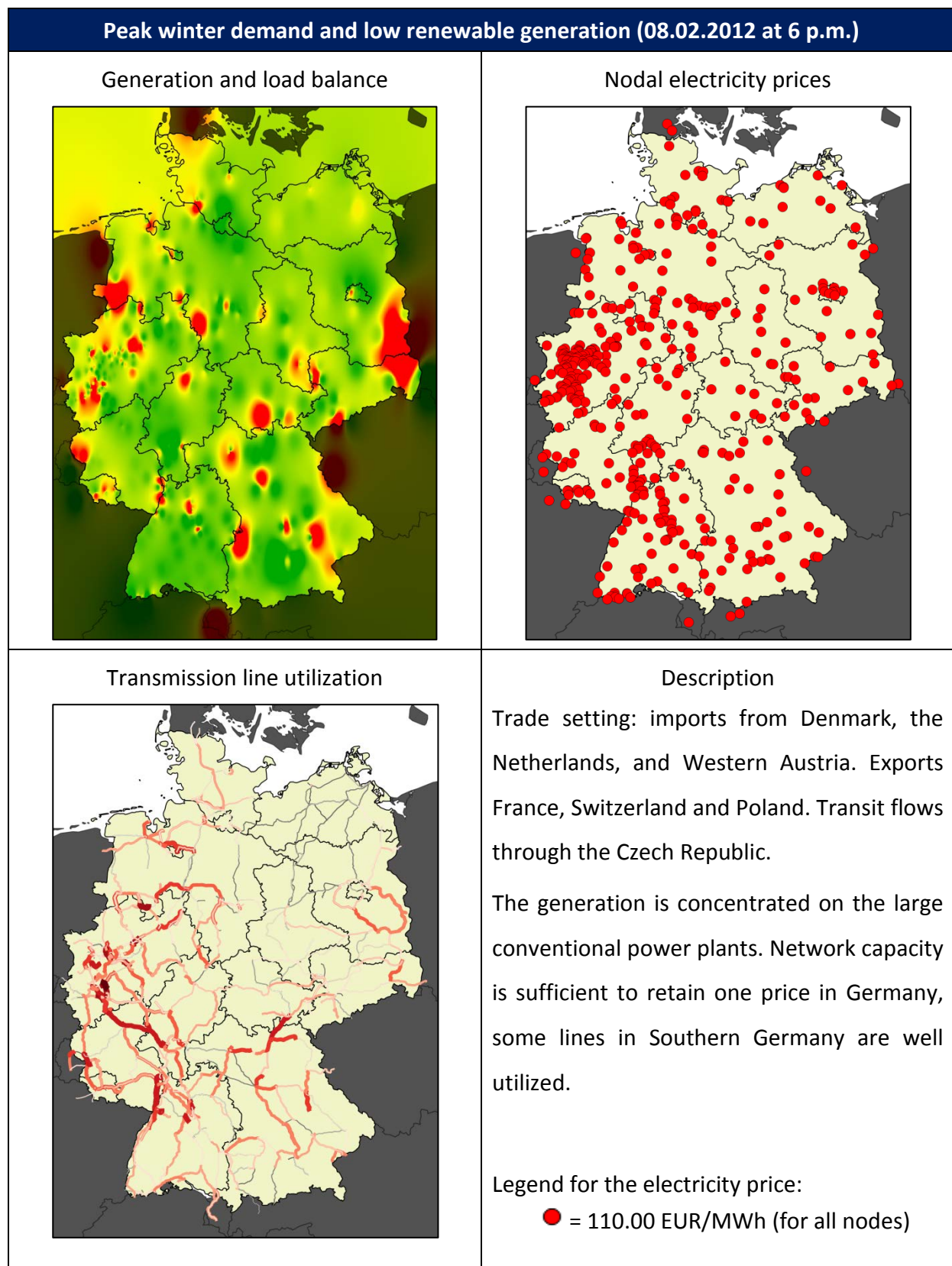
Figure 24: Snap shot of the system with peak load and low renewables
