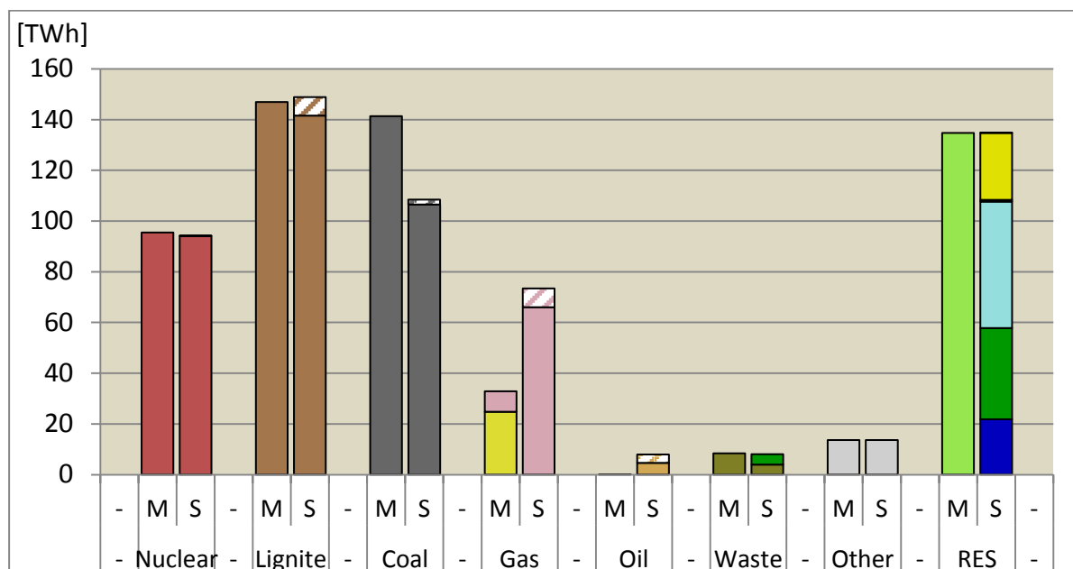
Figure 19: Generation quantities: Model results (M) compared to statistics (S)
