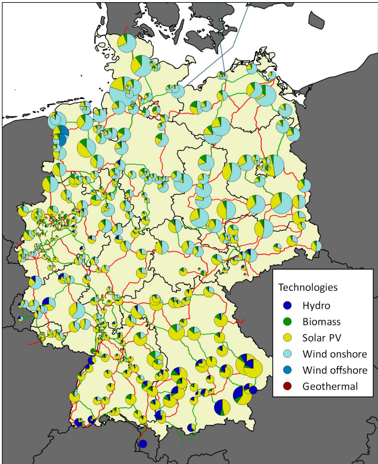
Figure 12: Renewable generation capacity on a nodal level
