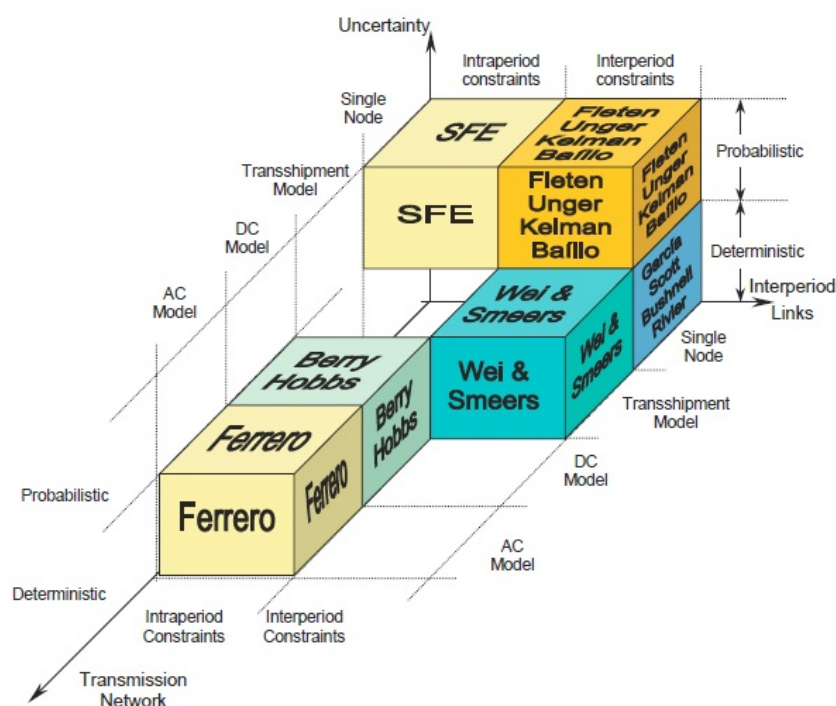
Figure 2: Characterization by uncertainty, transmission network, and interperiod links
