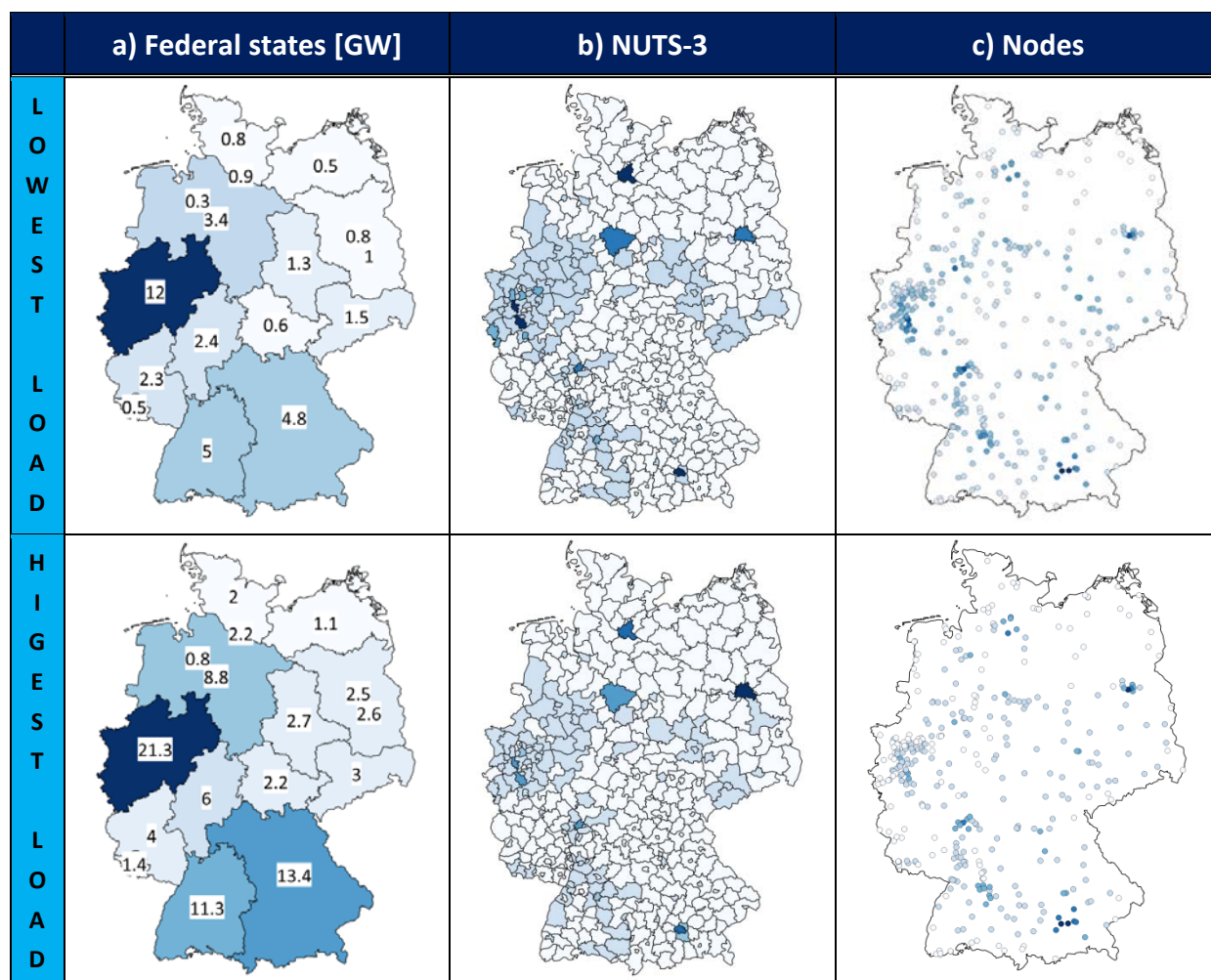
Figure 6: Stages of spatial load allocation
