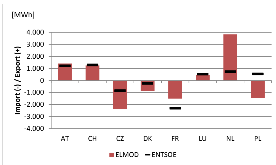
Figure 37: Cross-border flows from (+) and to (-) Germany
