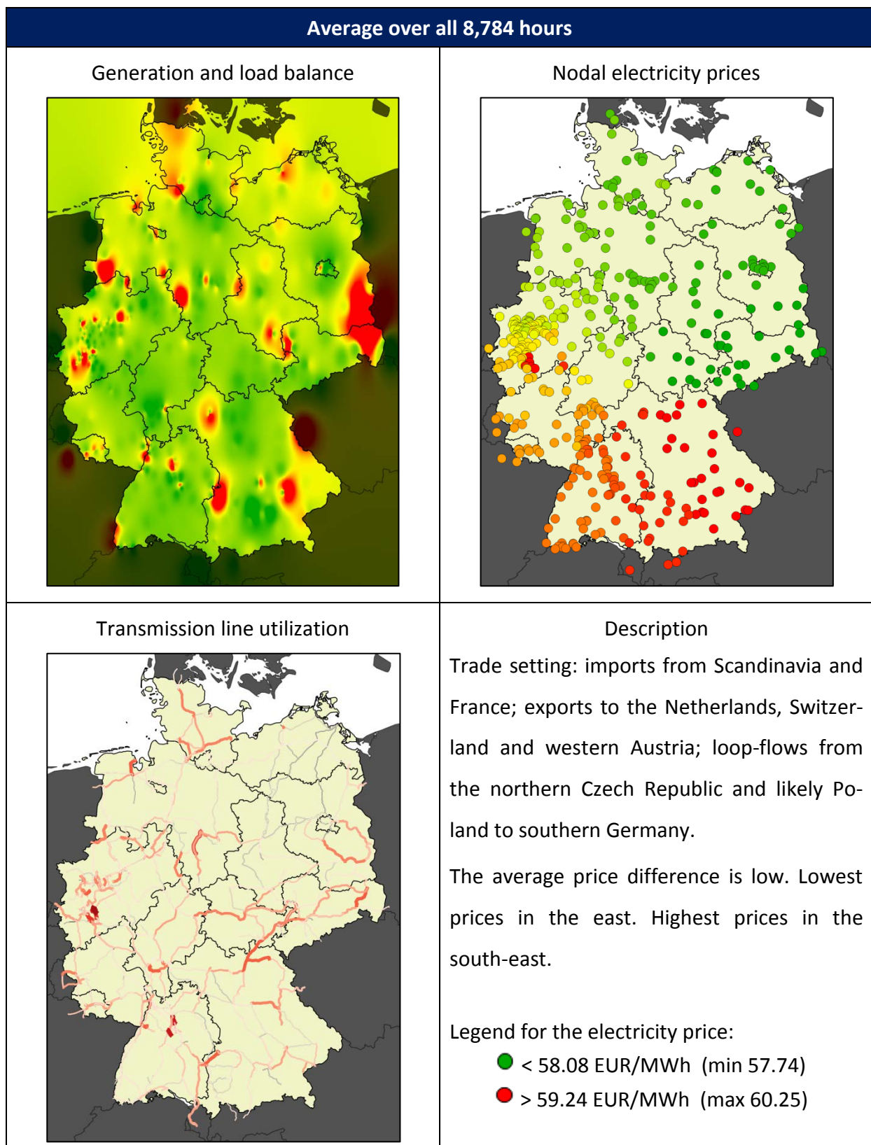
Figure 23: Snap shot of the system in average state of all hours
