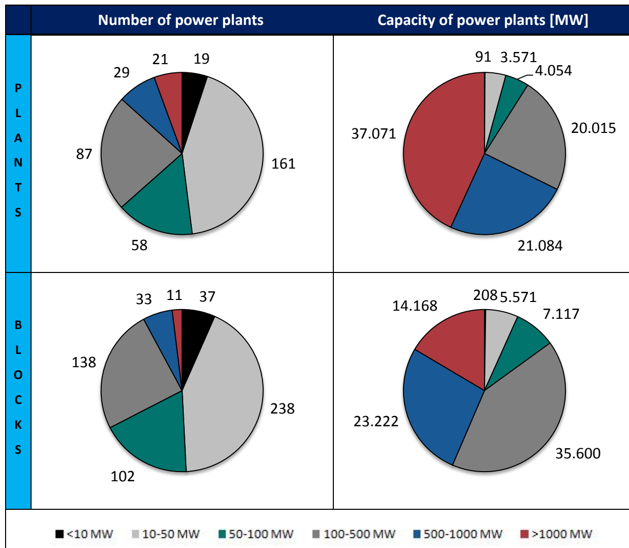
Figure 8: Comparison of number and capacity of conventional power plants 15
