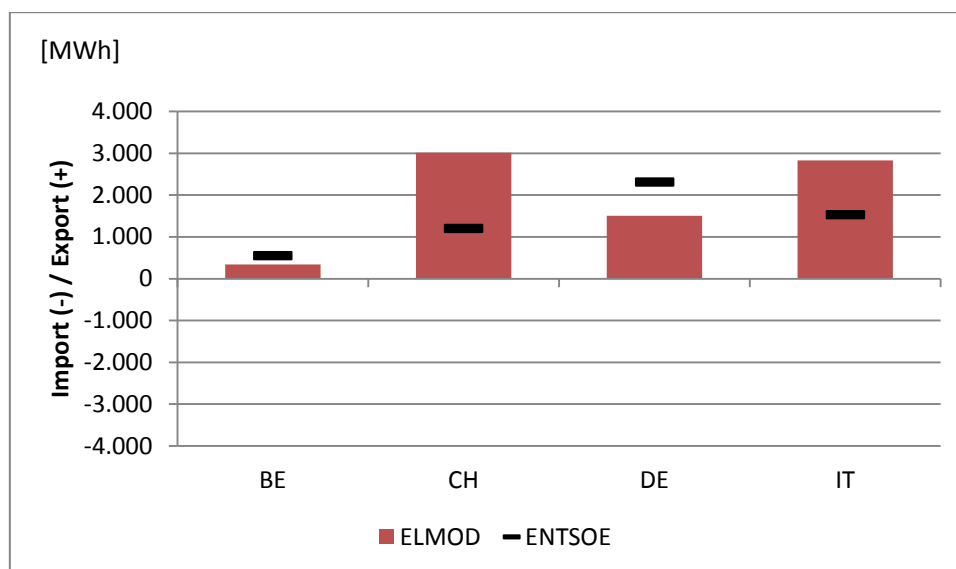
Figure 38: Cross-border flows from (+) and to (-) France
