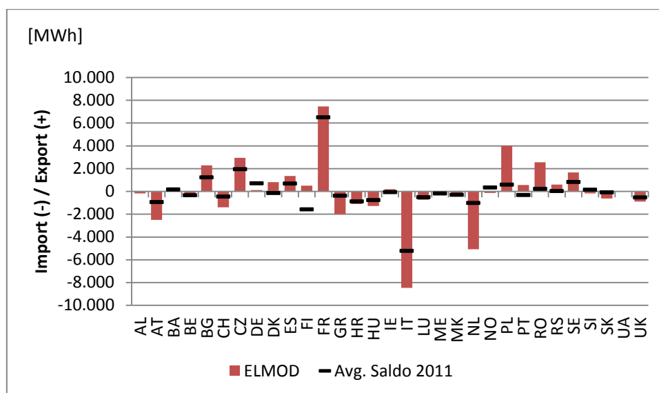
Figure 36: Average exchange saldo of European countries
