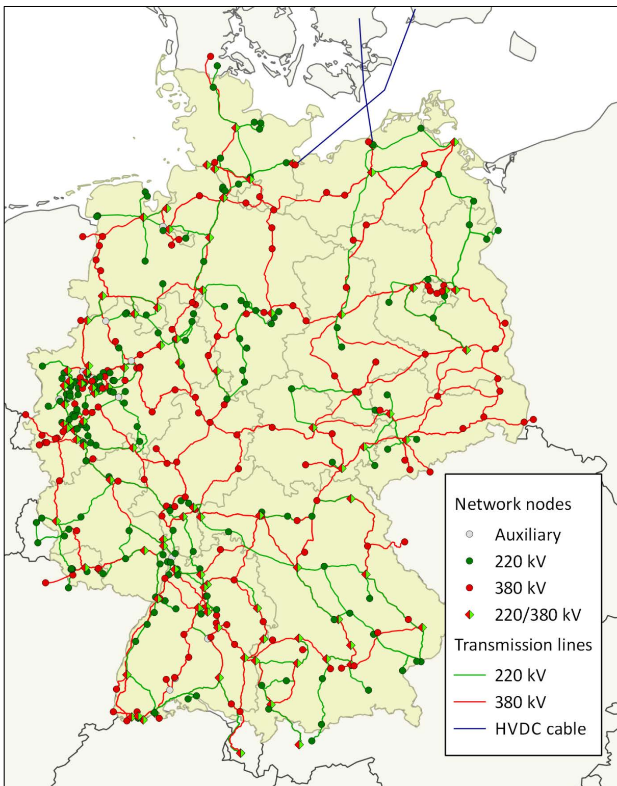
Figure 4: The German high-voltage electricity transmission system in 2012
