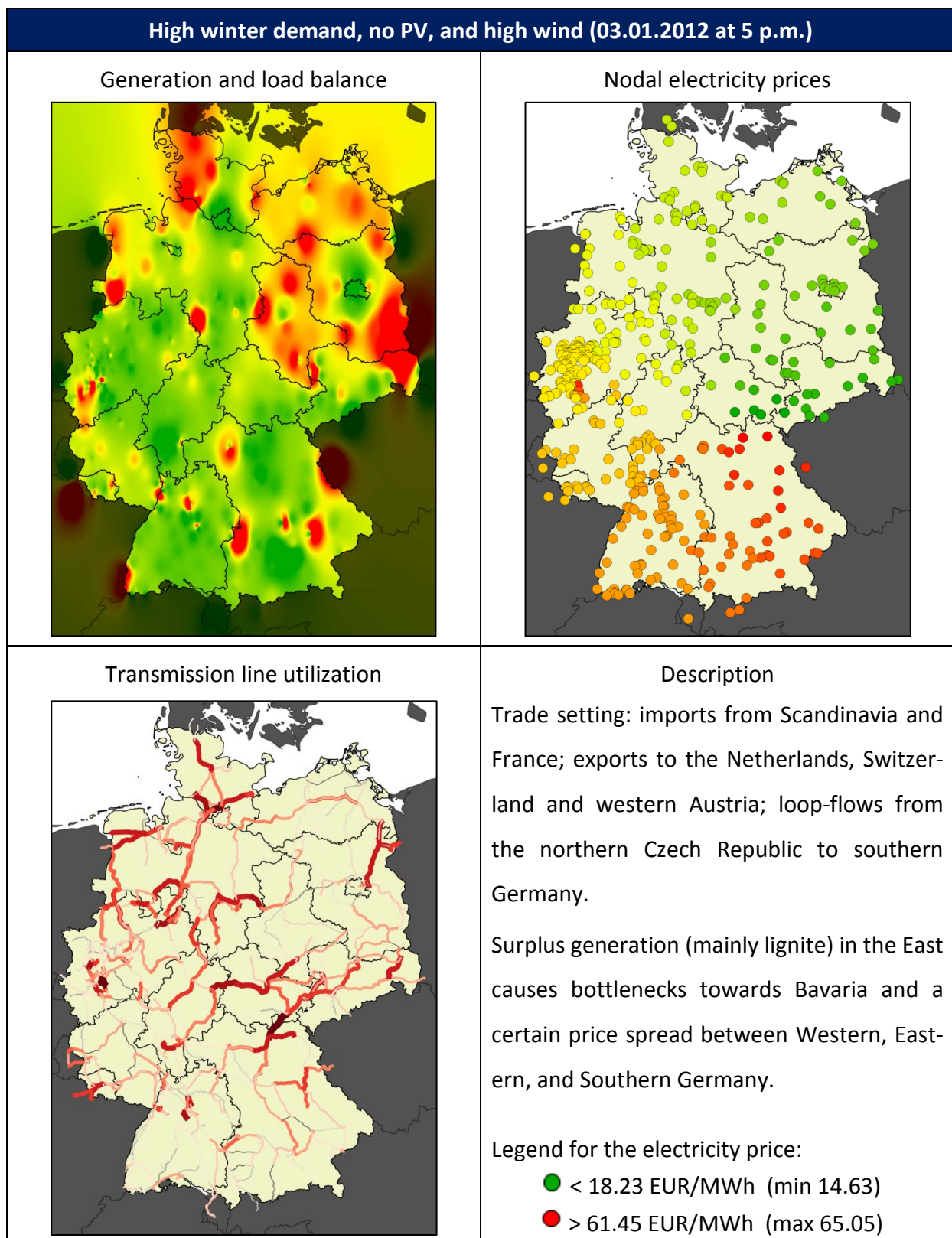
Figure 25: Snap shot of the system with high winter load and high wind generation
