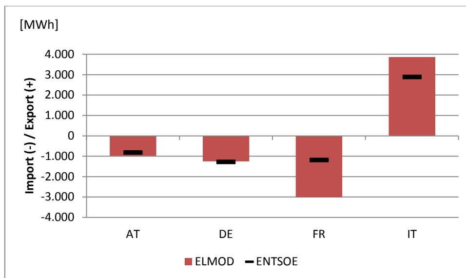
Figure 39: Cross-border flows from (+) and to (-) Switzerland
