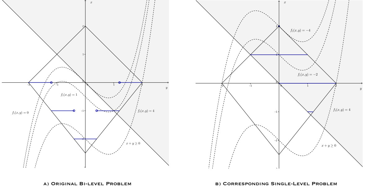
FIGURE 7. A Mixed-Integer Nonlinear Bi-level Programming Problem
