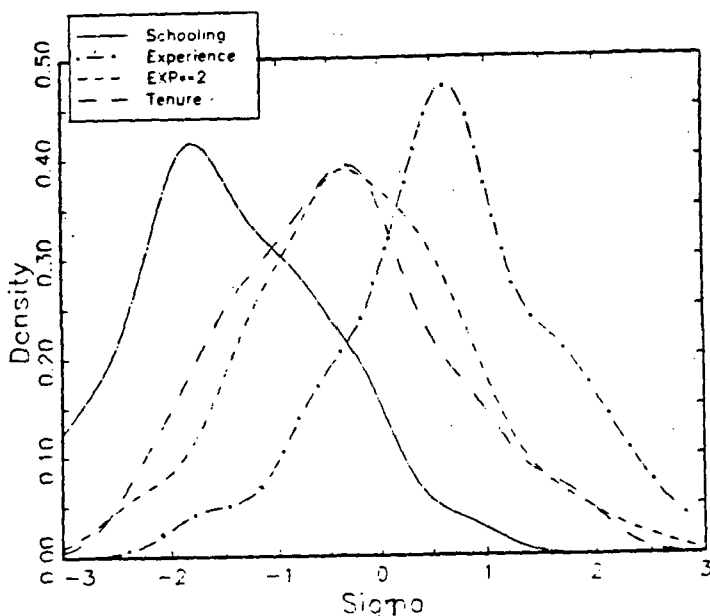
Figure 5: The distribution of \hat{\beta}_S - \hat{\beta}_S for the coefficients: Schooling , Experience , Exp.* Exp. and Tenure . Kernel density estimate on the basis of 100 replications of the artificial attrition experiment.
