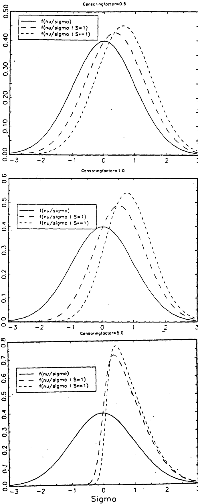
Figure 3: Comparison of the unselected distribution of \nu_{i,t} with the censored distributions \nu_{i,t} | S_{i,t} and \nu_{i,t} | S_{i,t}^* for f=0.5, 1 and 5 .
