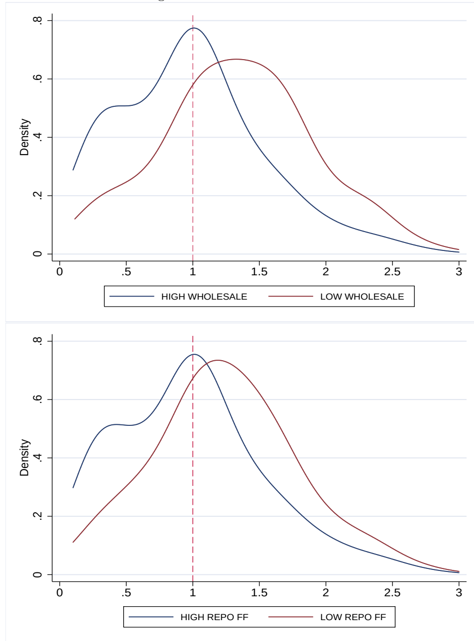
Figure 1: KERNEL DENSITIES
