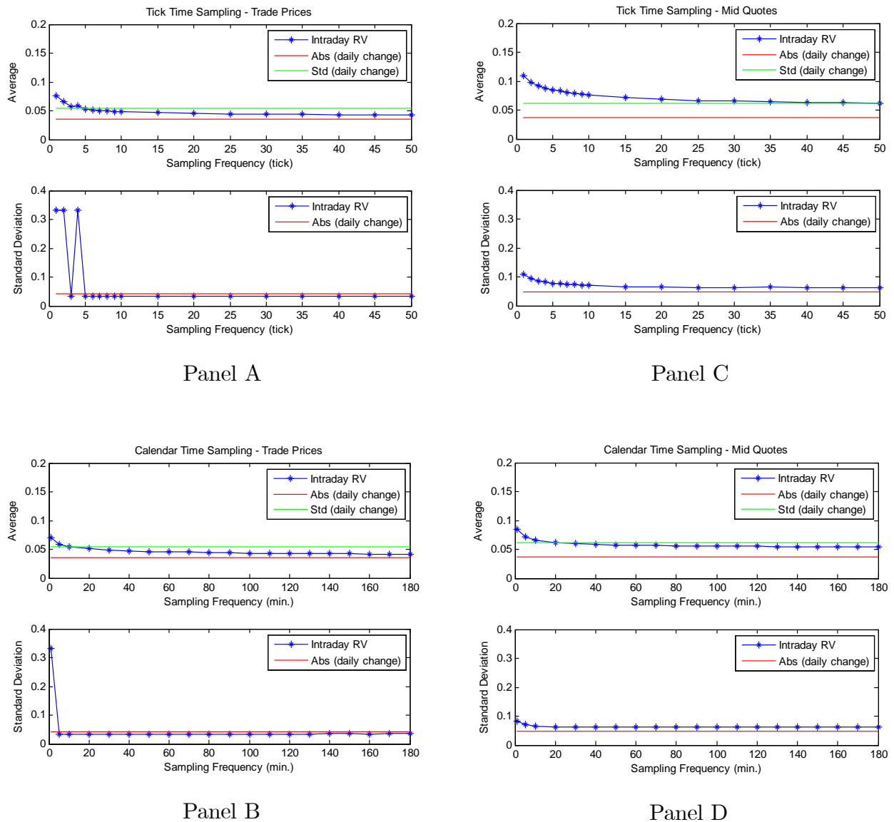
Figure 8: Volatility signature
