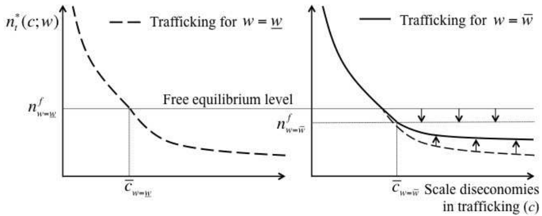
Figure 4: This figure shows that an increase in female wages from \underline{w} (left graph) to \bar{w} (right graph) weakly decreases total prostitution but weakly increases trafficking.
