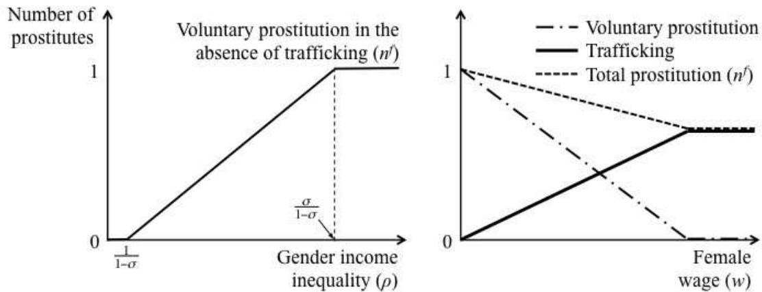
Figure 2: The left graph shows how the male-female income ratio \rho affects voluntary prostitution in the absence of trafficking. The right graph shows how the female wage w affects trafficking.
