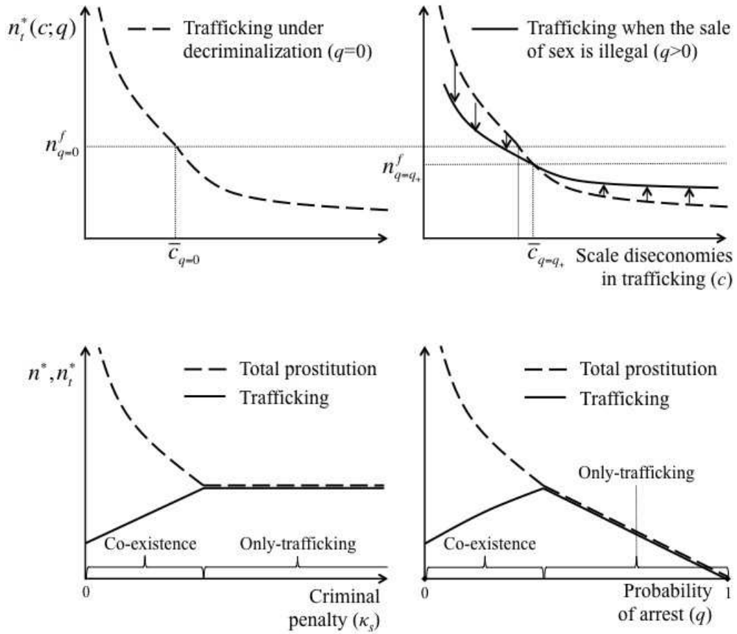
Figure 5: The top row shows how a change from decriminalization (left graph) to criminalizing prostitutes (right graph) affects trafficking. The bottom row shows how trafficking and total prostitution vary with the criminal penalty \kappa_s (left graph) and the arrest probability q (right graph) when prostitutes are criminalized.
