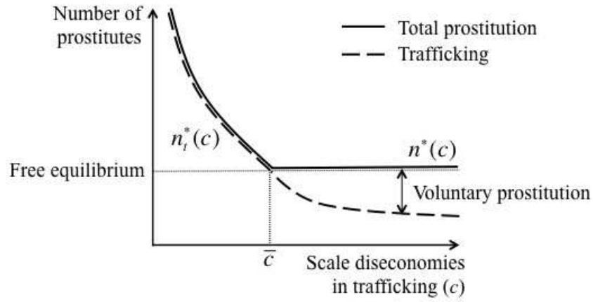
Figure 3: This graph shows how changes in the costliness of trafficking affect the total level of prostitution as well as its decomposition into voluntary prostitution and trafficking.
