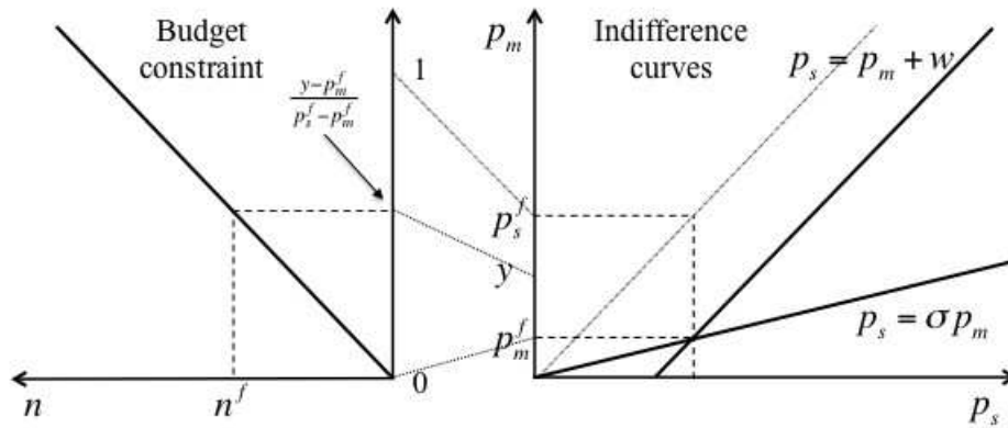
Figure 1: This figure shows the equilibrium in the absence of trafficking. The indifference curves in the right graph determine the prices of sex and marriage. Given these prices, the left graph uses the budget constraint to determine the supply of voluntary prostitution.
