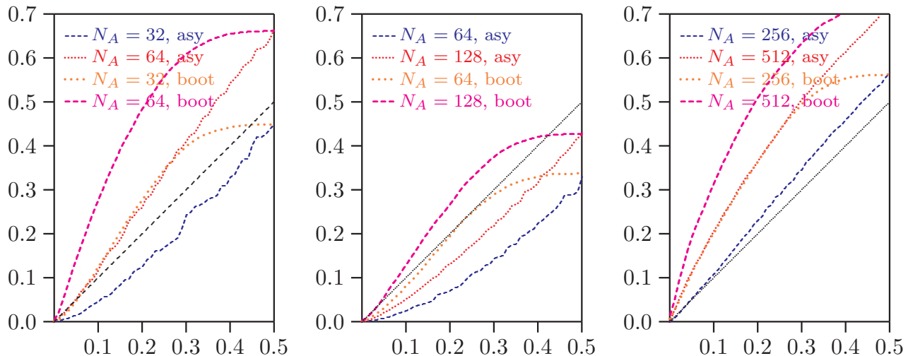
Figure 5: Power curves, z^- = 0.1
